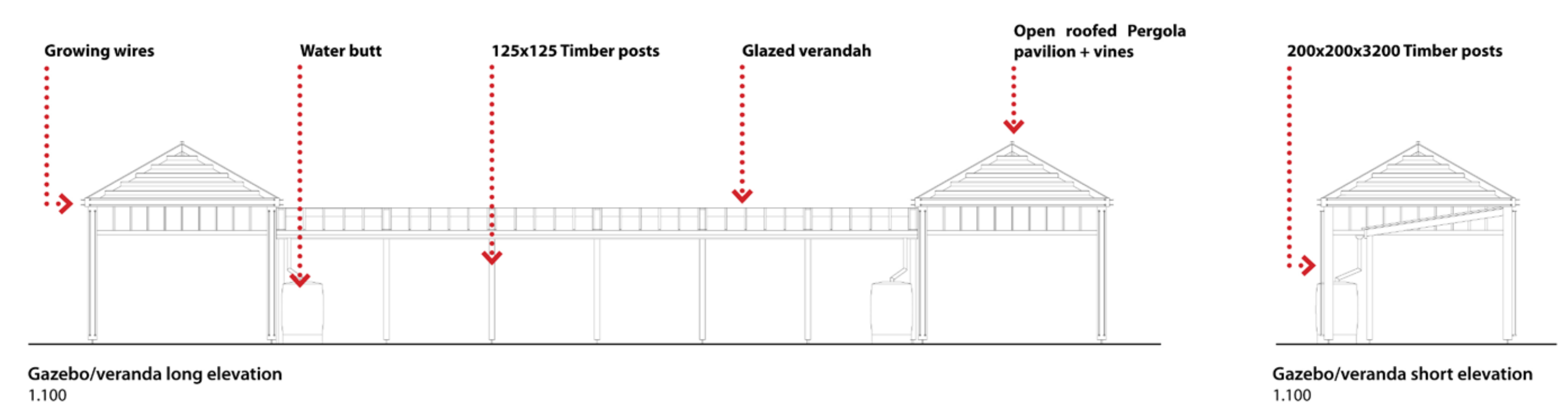
Two timber pergola pavilions and a glazed verandah 1:100
