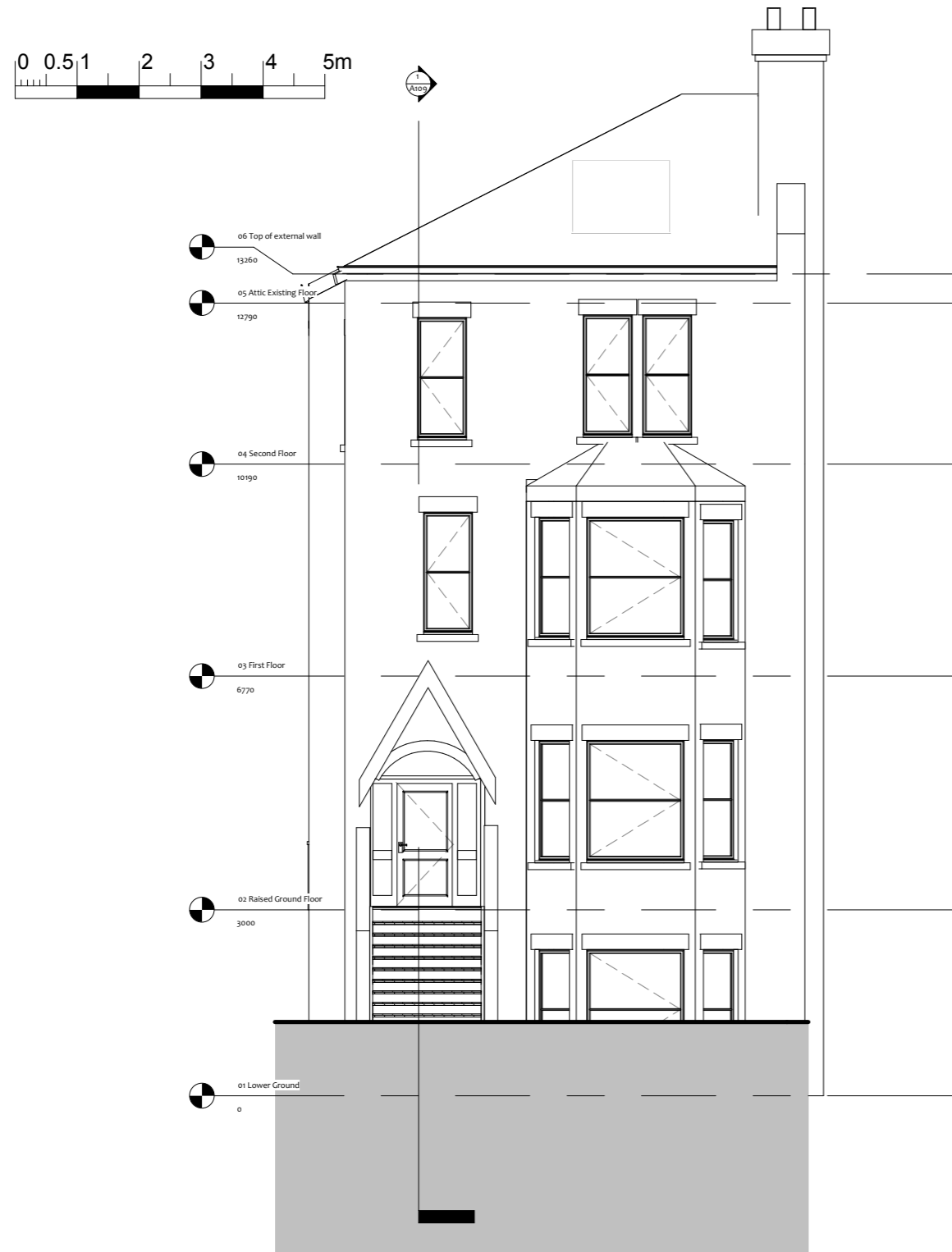
Front Elevation 1 : 100
