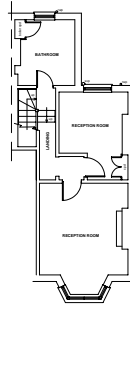
EXISTING RAISED GROUND FLOOR PLAN
