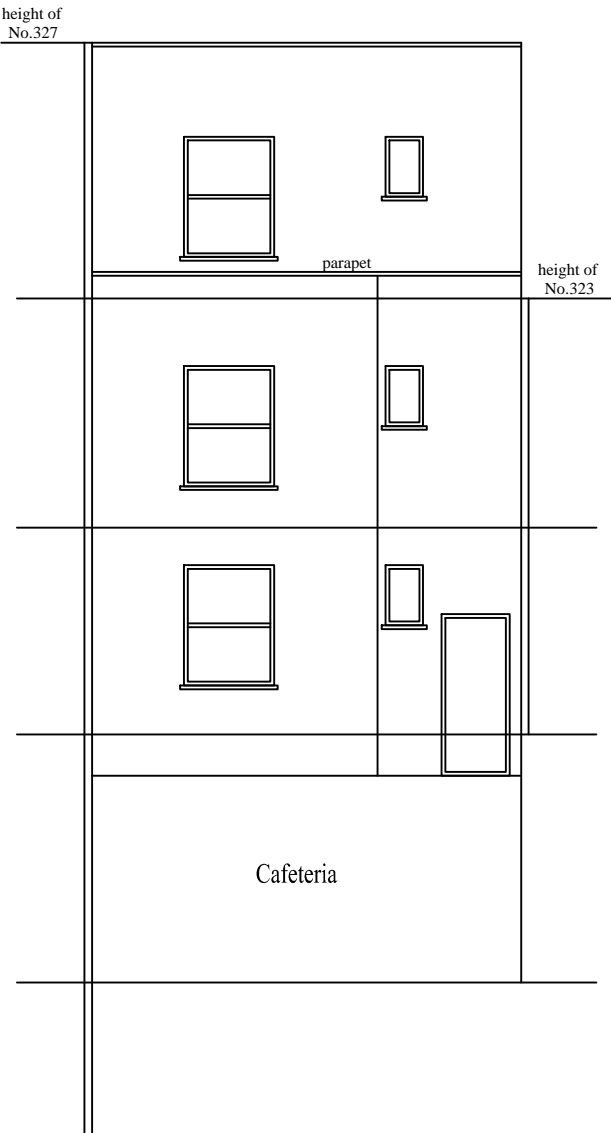
PROPOSED BB ELEVATION (REAR)
