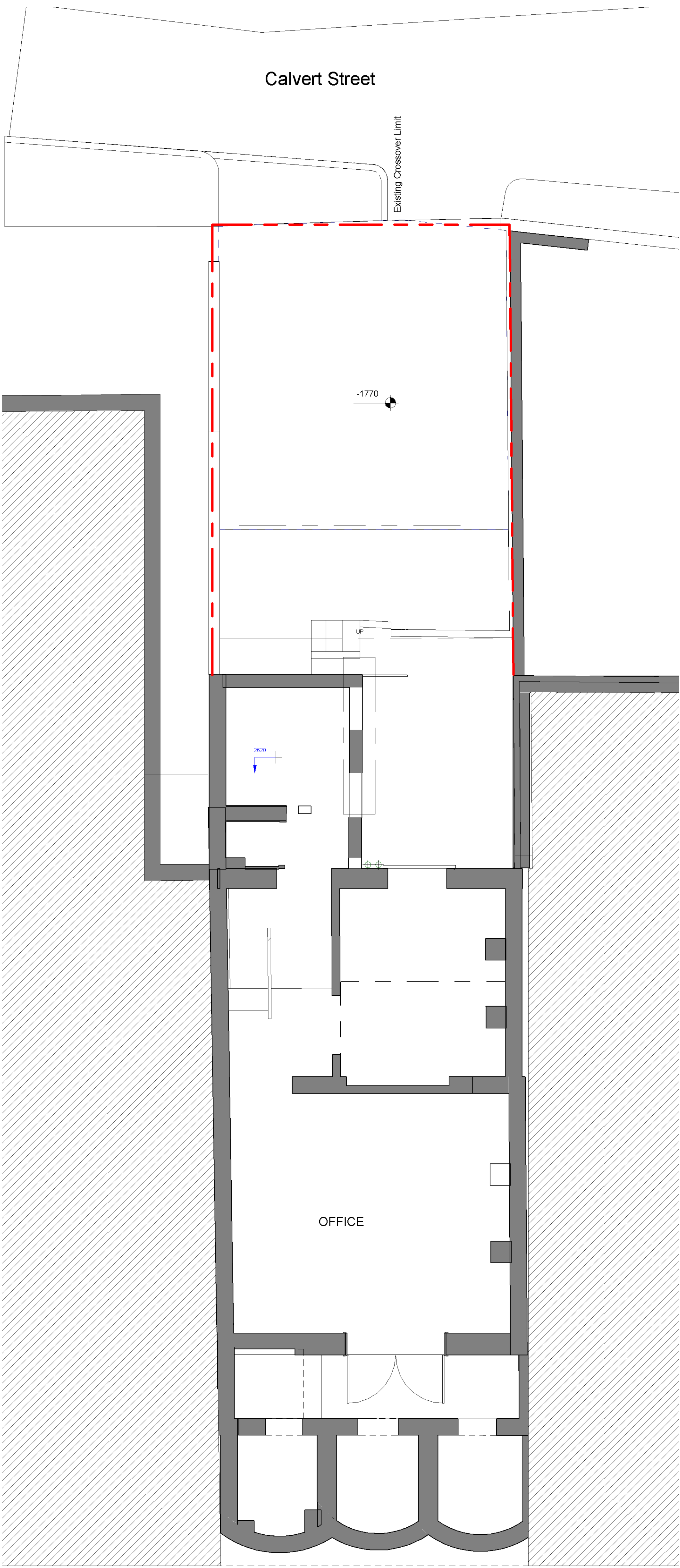
Existing Lower Ground Floor Level 1 : 50
