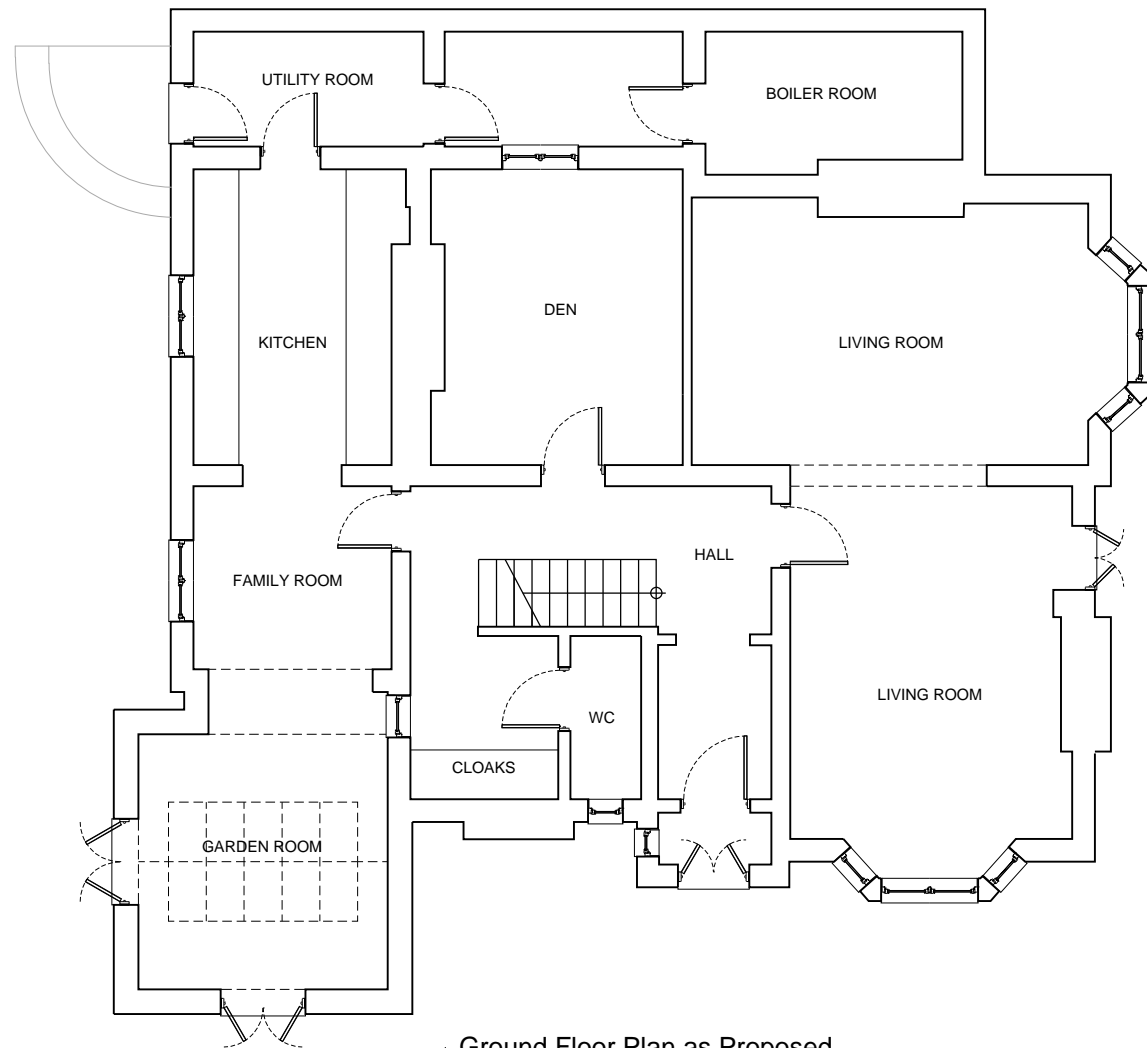
Ground Floor Plan as Proposed
