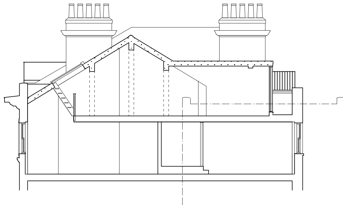
SECTION 1-1 (third and fourth floors)
