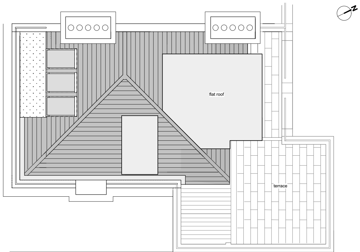
ROOF PLAN
