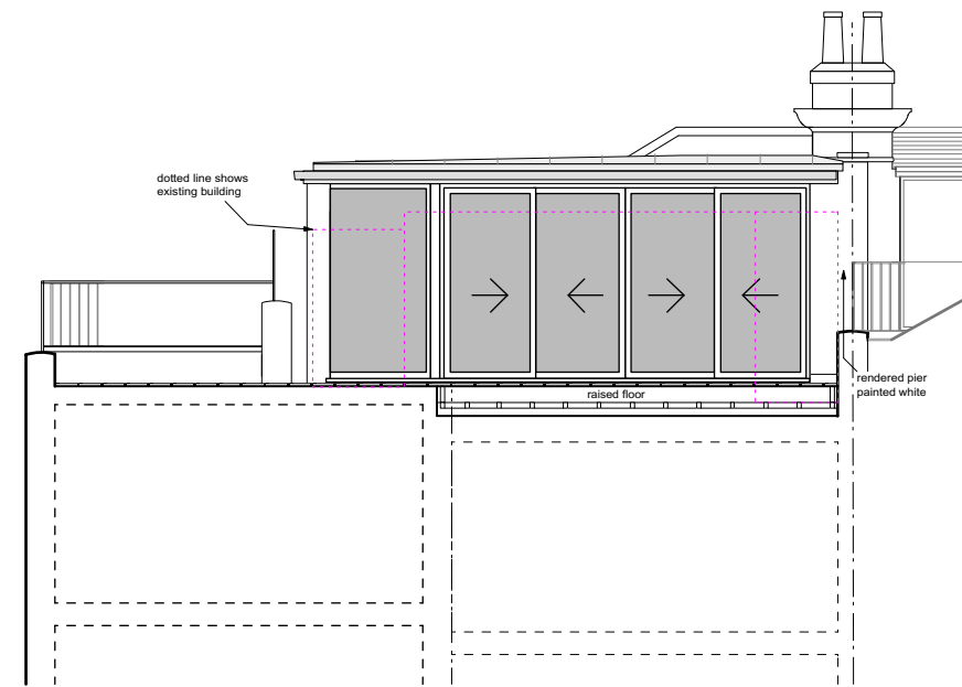
REAR ELEVATION
