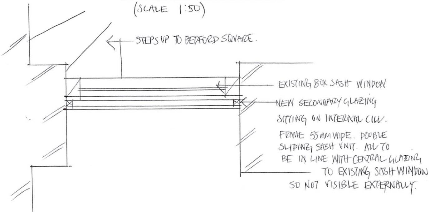
SECTION A-A THROUGH EXISTING WINDOW TO SHOW LOCATION OF SECONDARY GLAZING.
