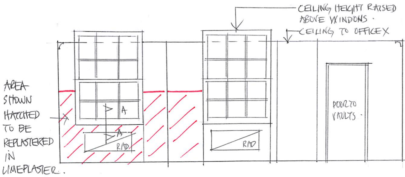
ELEVATION OF WINDOWS TO ARCHIVE OFFICE X (SCALE 1:50)
