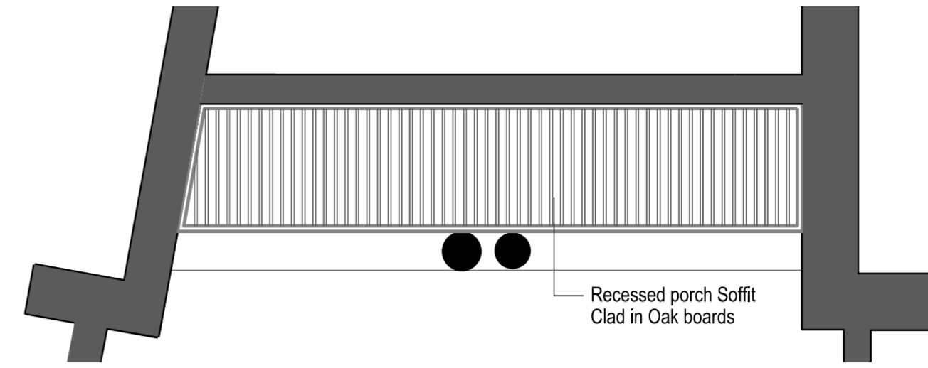
PORCH- REFLECTED CEILING PLAN
