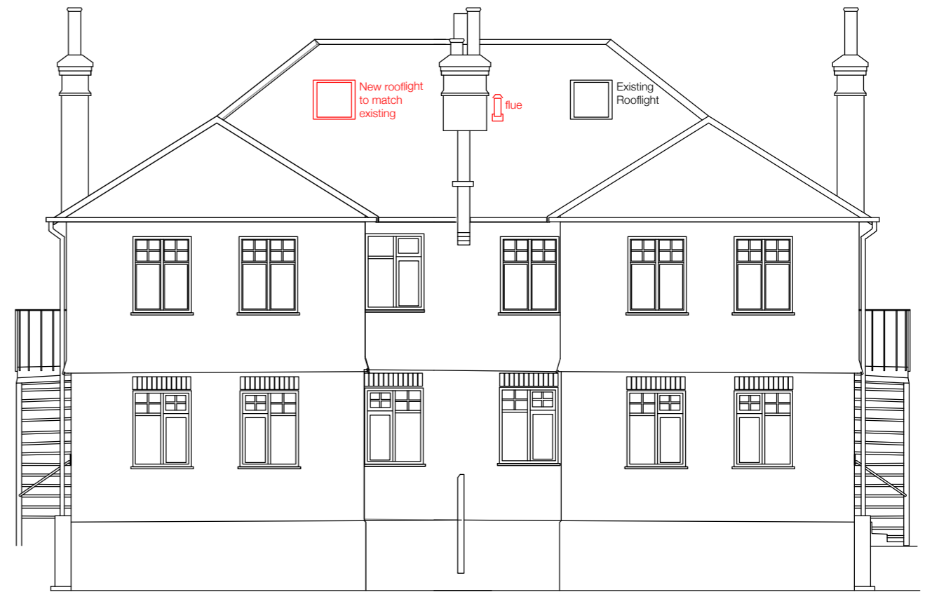
West Elevation (Garden) (proposal in red)
