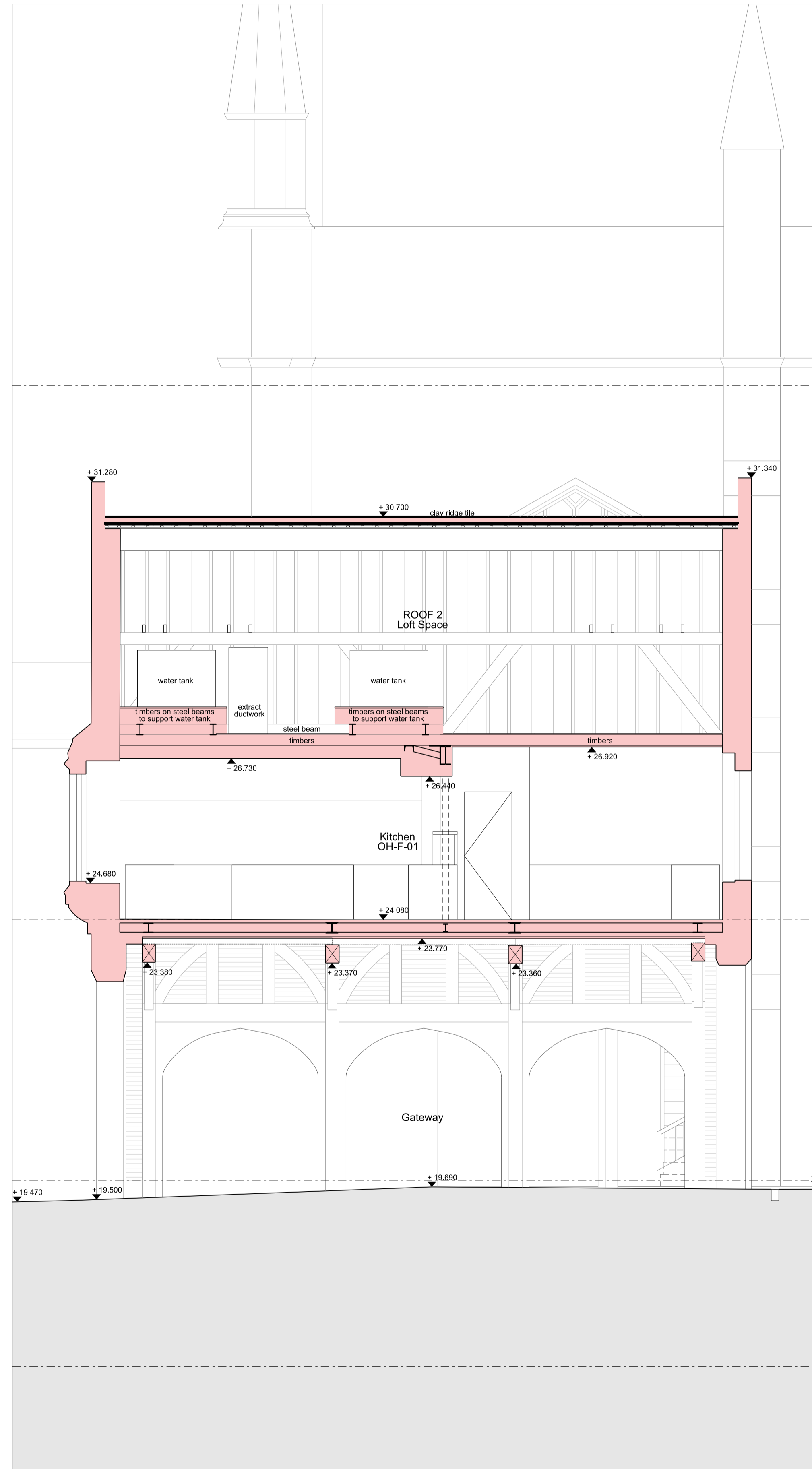
Existing Section A-A
