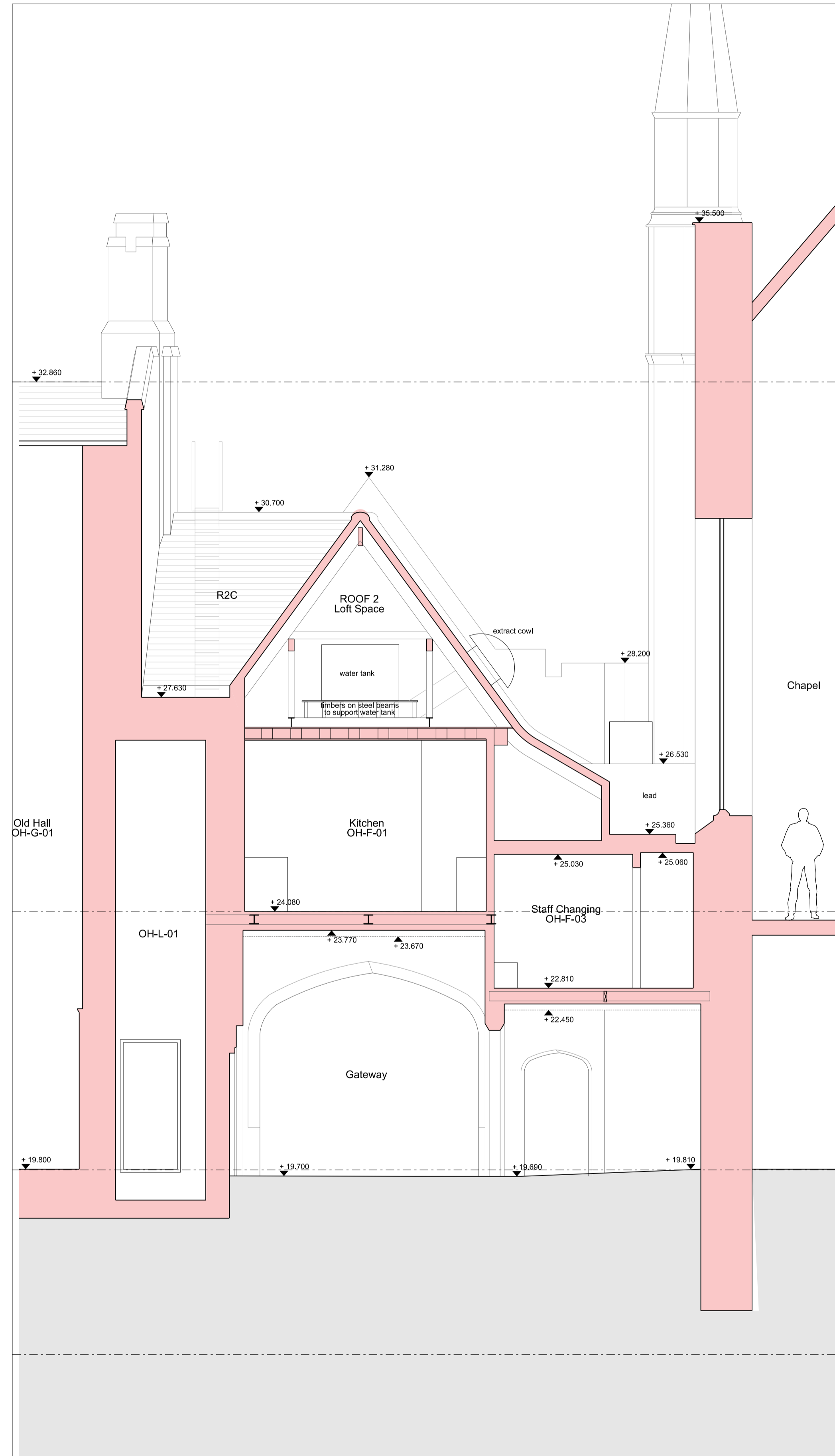
Existing Section C-C
