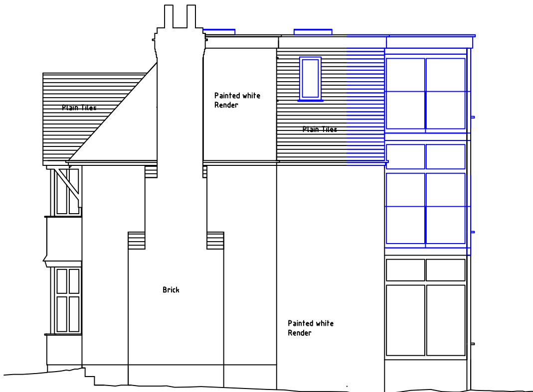
West Elevation
