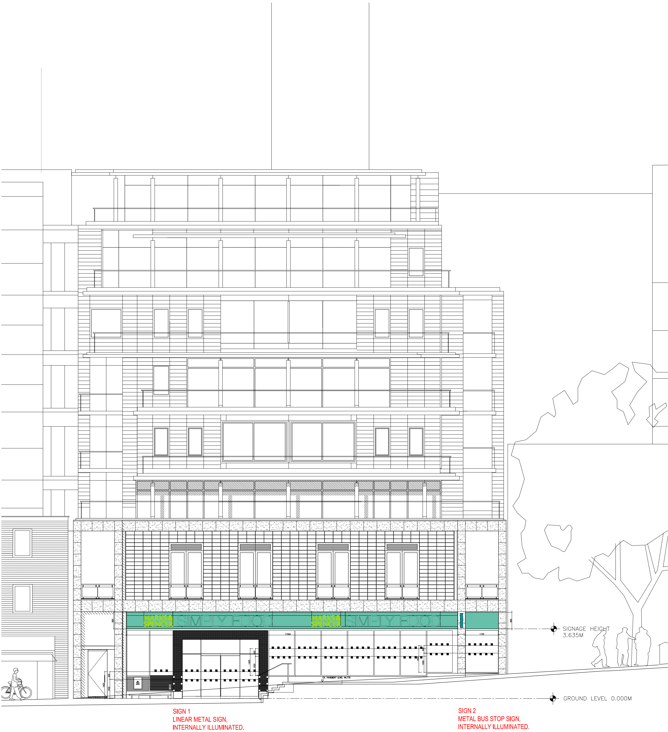
EXISTING ELEVATION A SCALE 1:100 @ A1
