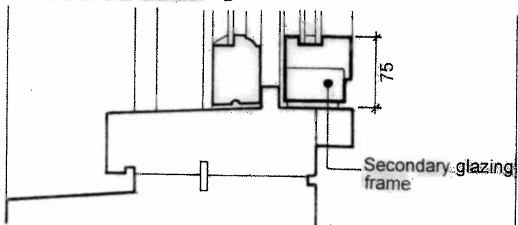
Detail Section B
