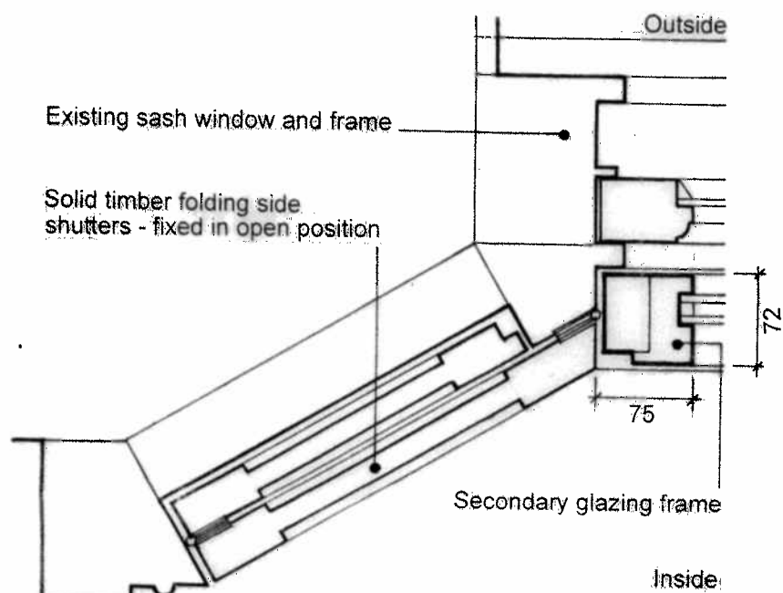
Detail Plan A
