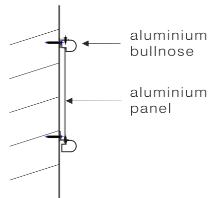
SIGN C - scale 1:10
