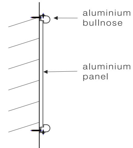
SIGN D - scale 1:10
