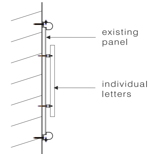
SIGN H - scale 1:10
