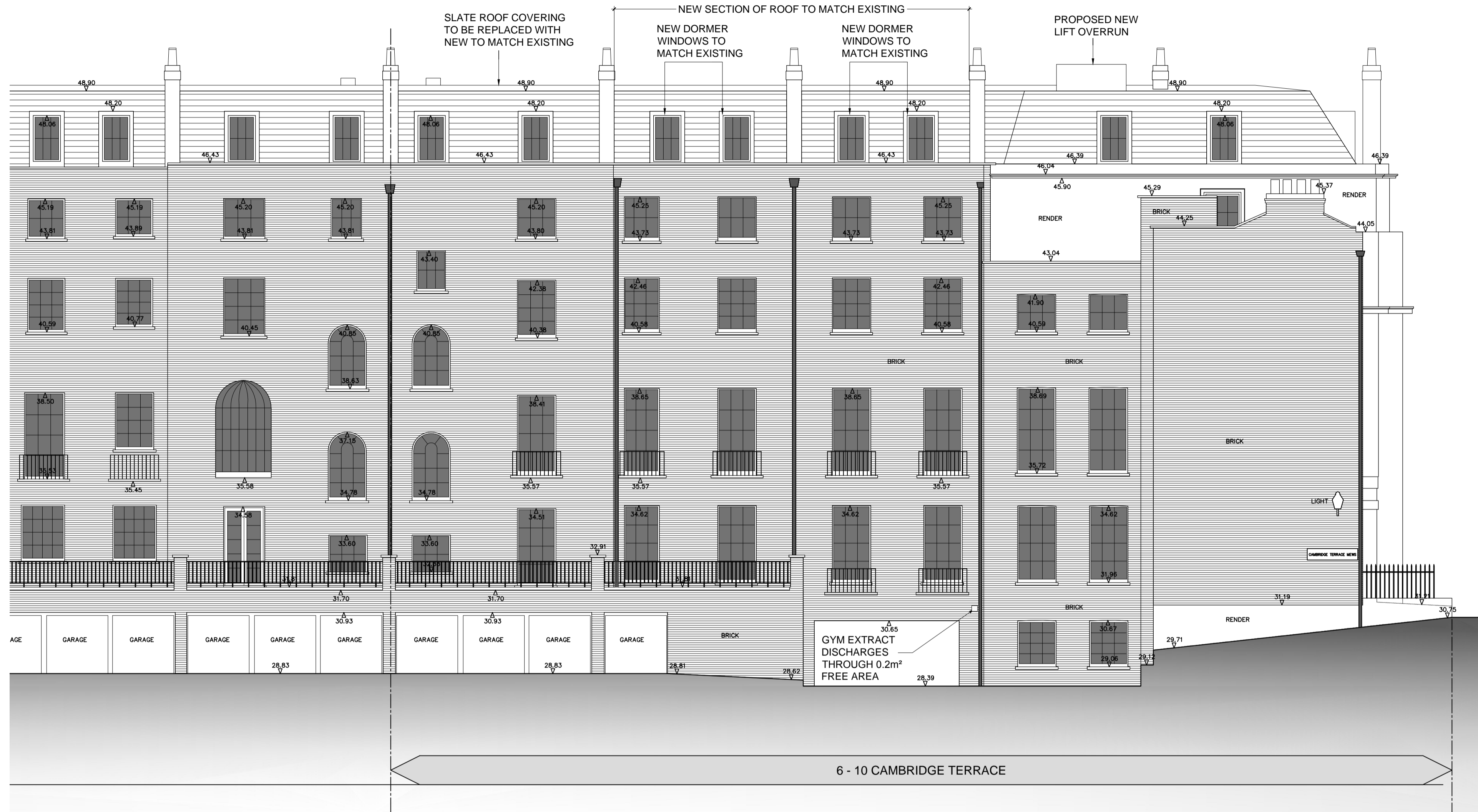
CAMBRIDGE TERRACE REAR ELEVATION
