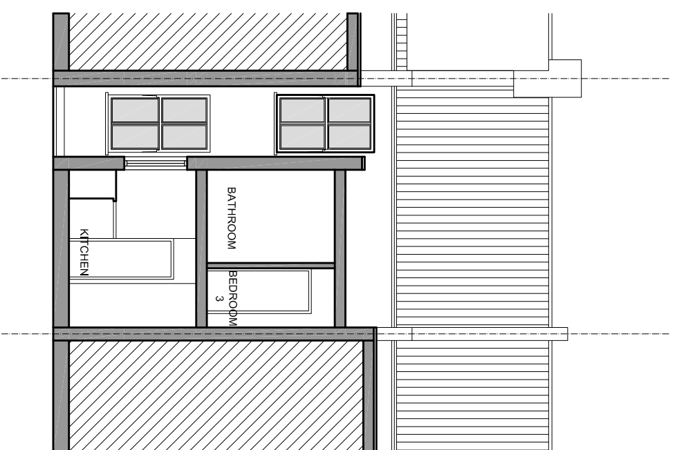
SECTION BB 0 1 2 3 METRES
