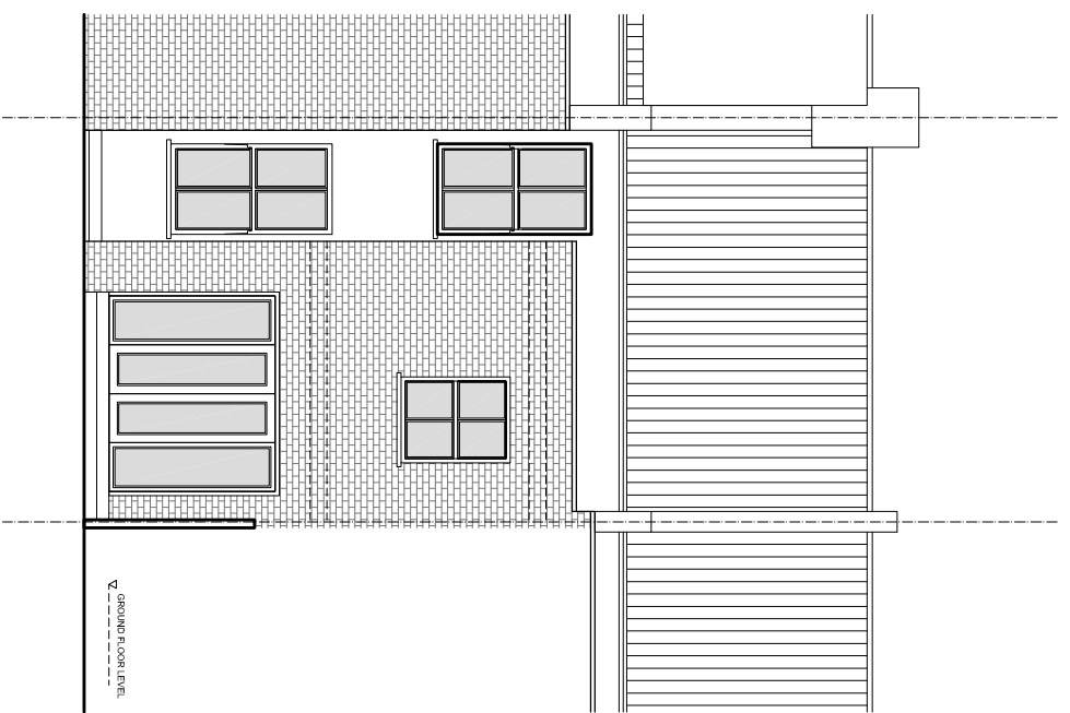
REAR ELEVATION 0 1 2 3 METRES
