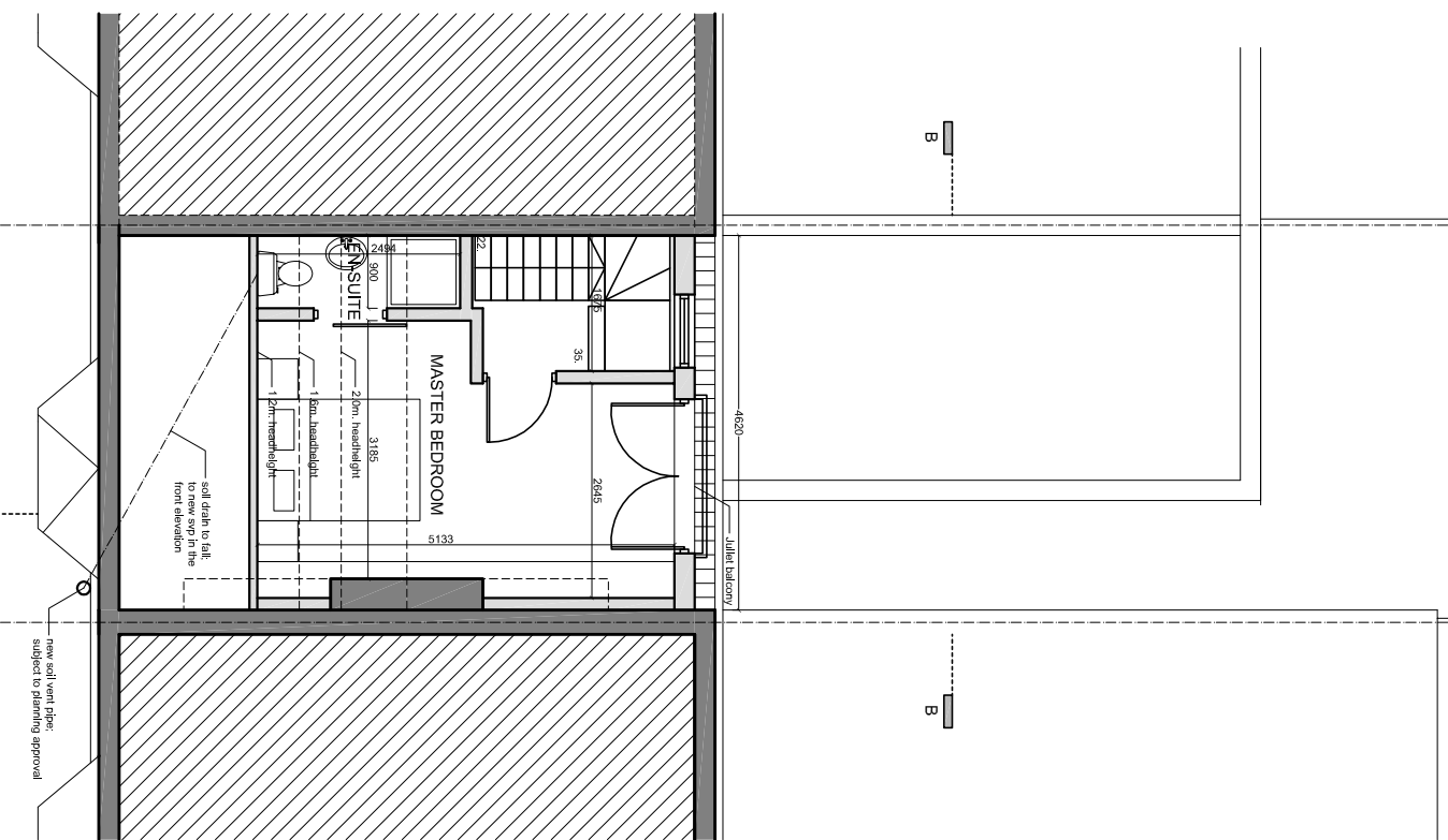
LOFT FLOOR PLAN
