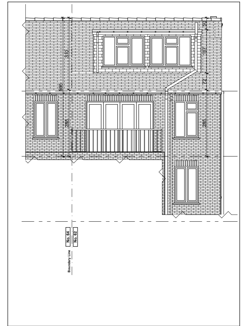
REAR ELEVATION
