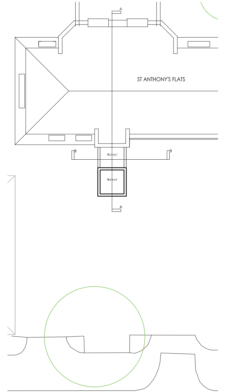
ROOF PLAN
