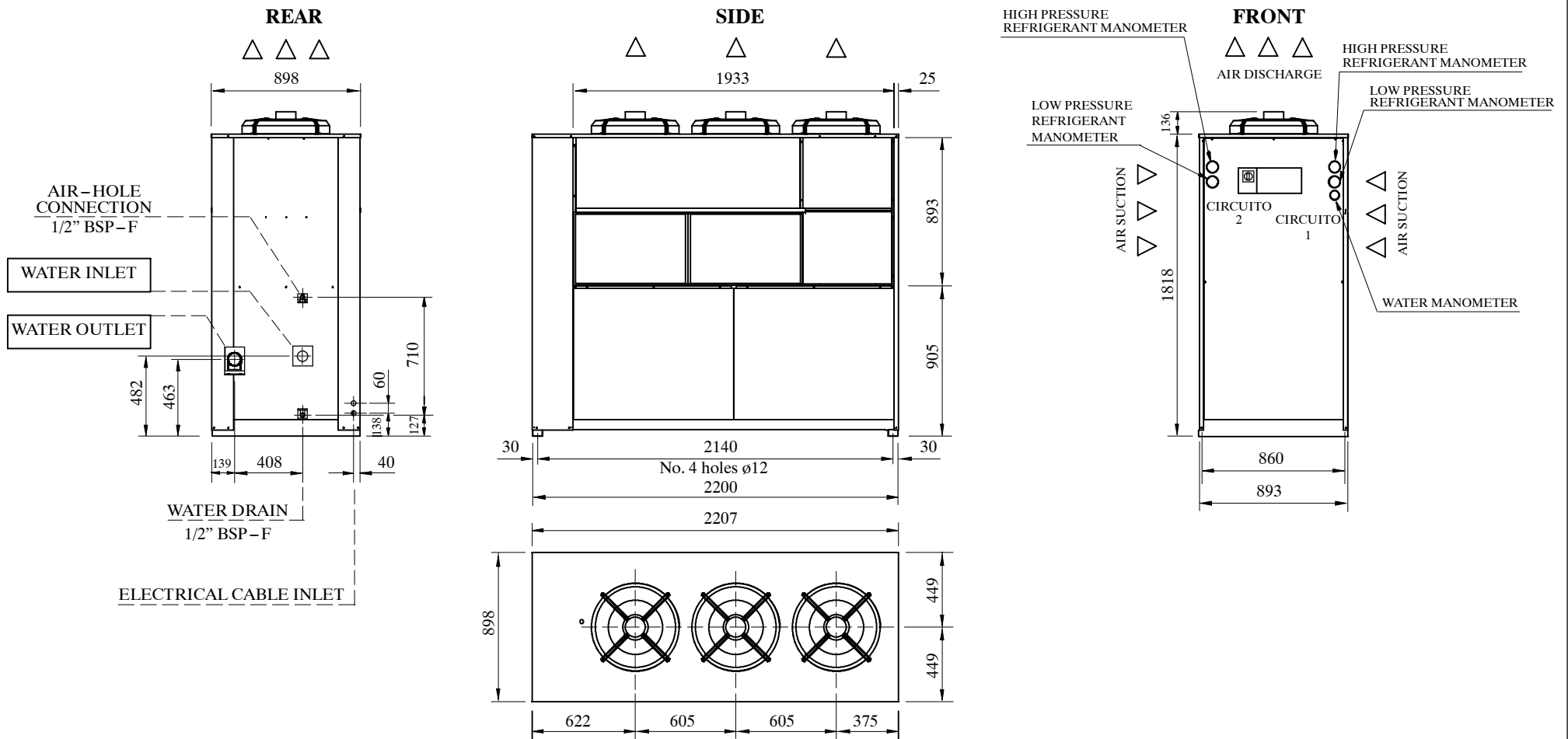
Fig. 2 Overall dimensions (ICE076–116)
