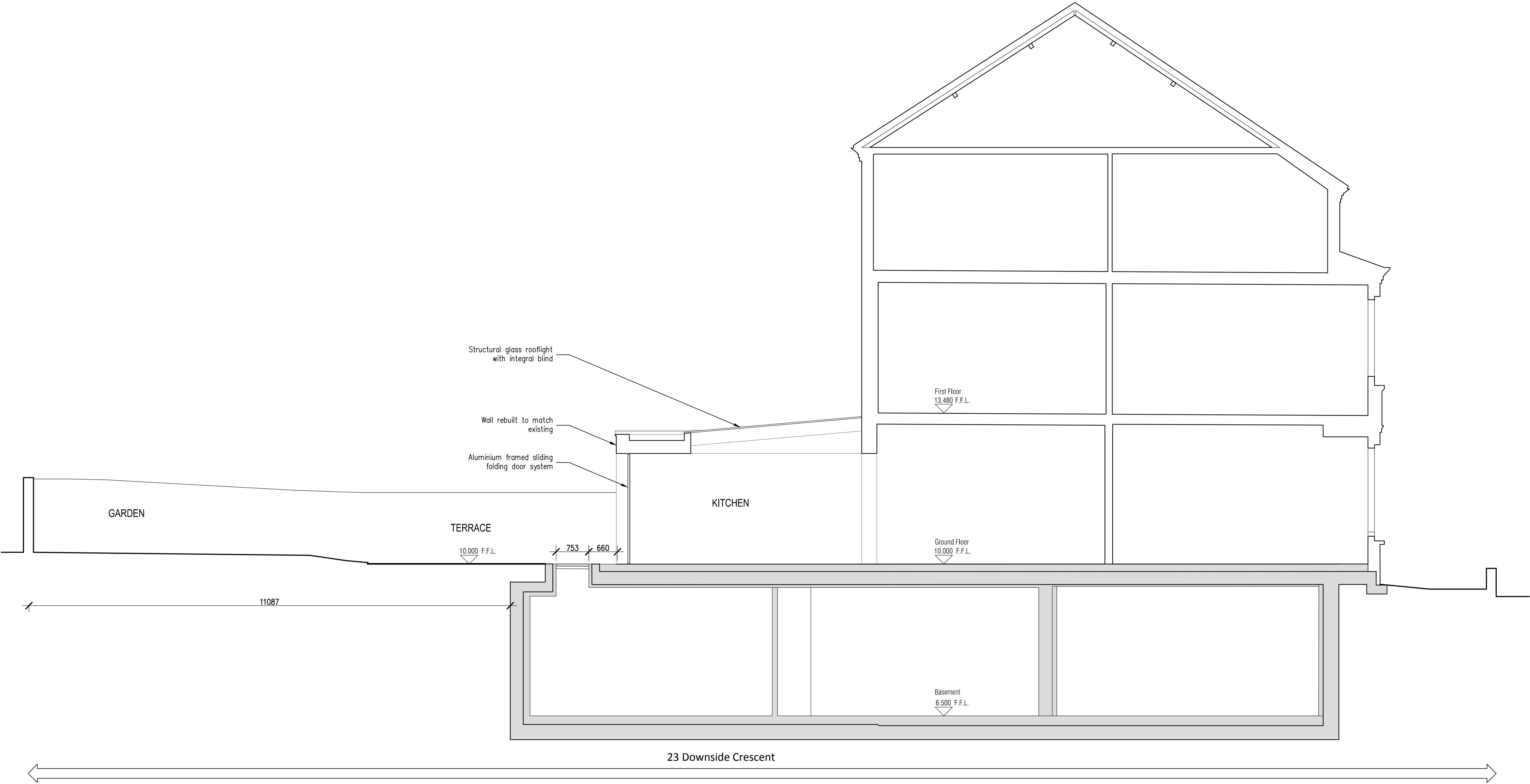
PROPOSED SECTION AA Scale 1:50@A1
