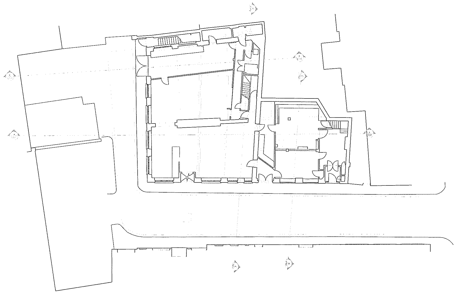
GROUND FLOOR 01
