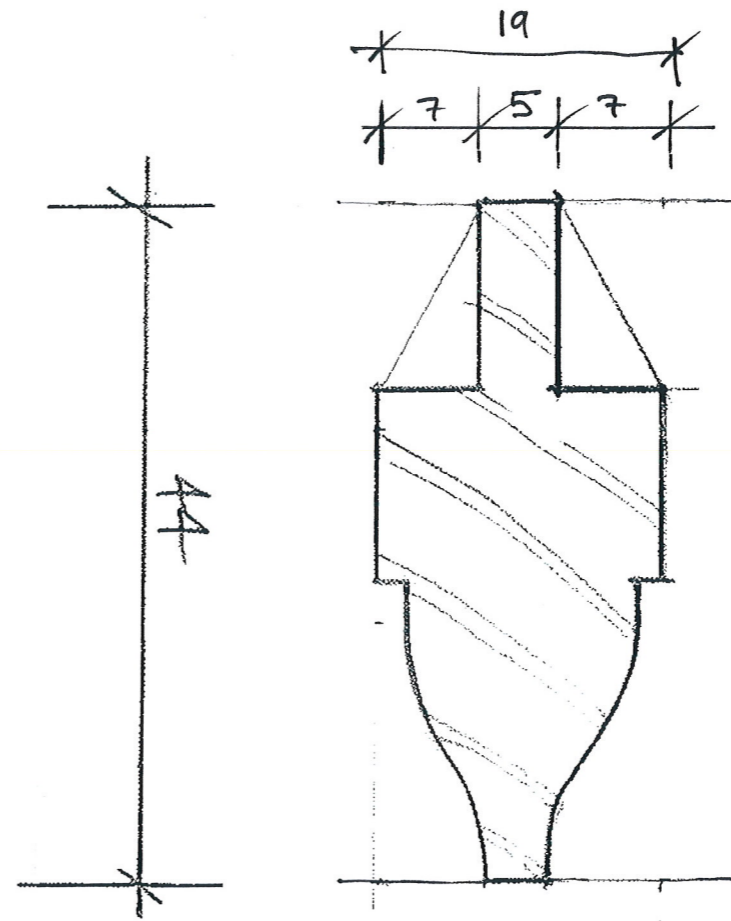
FRENCH DOOR GLAZING BARS 2:1
