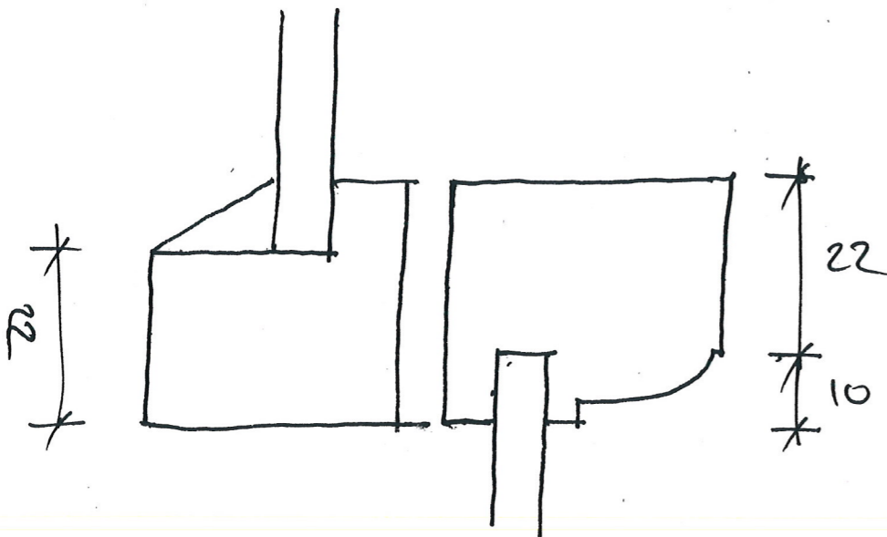
MEETING RAIL DETAIL (NTS)
