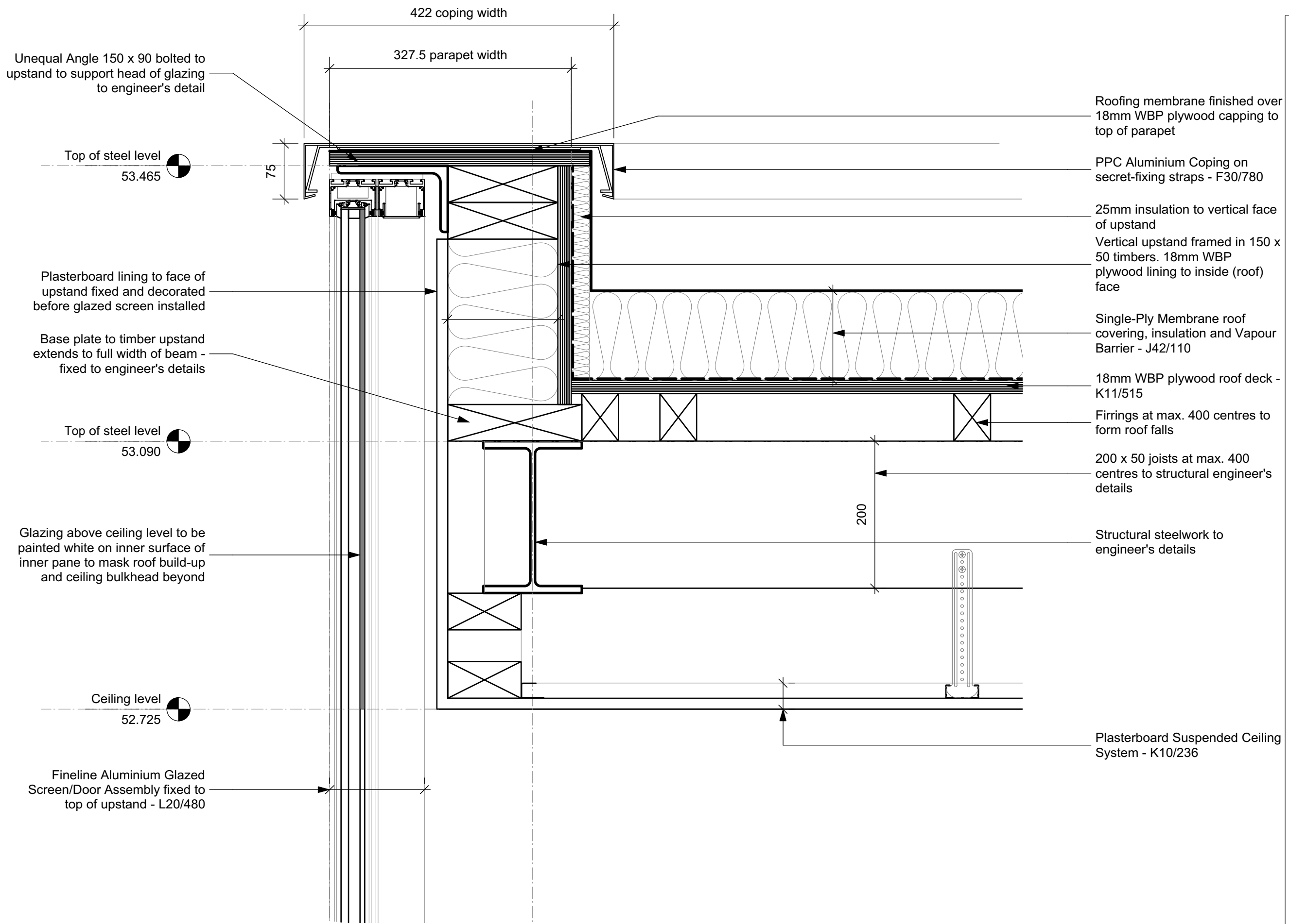
1 Glazed Screen Head Detail - Grid A D 527 Scale: 1:5
