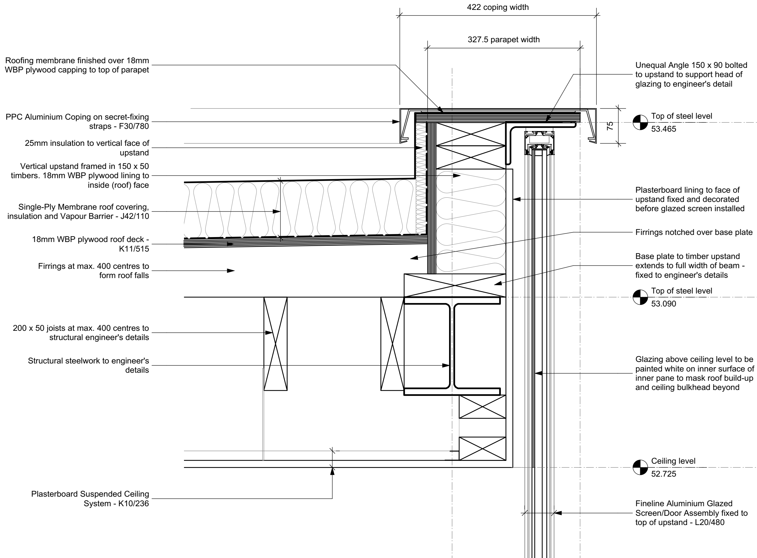
1 Glazed Screen Head Detail - Grid 1 D 526 Scale: 1:5
