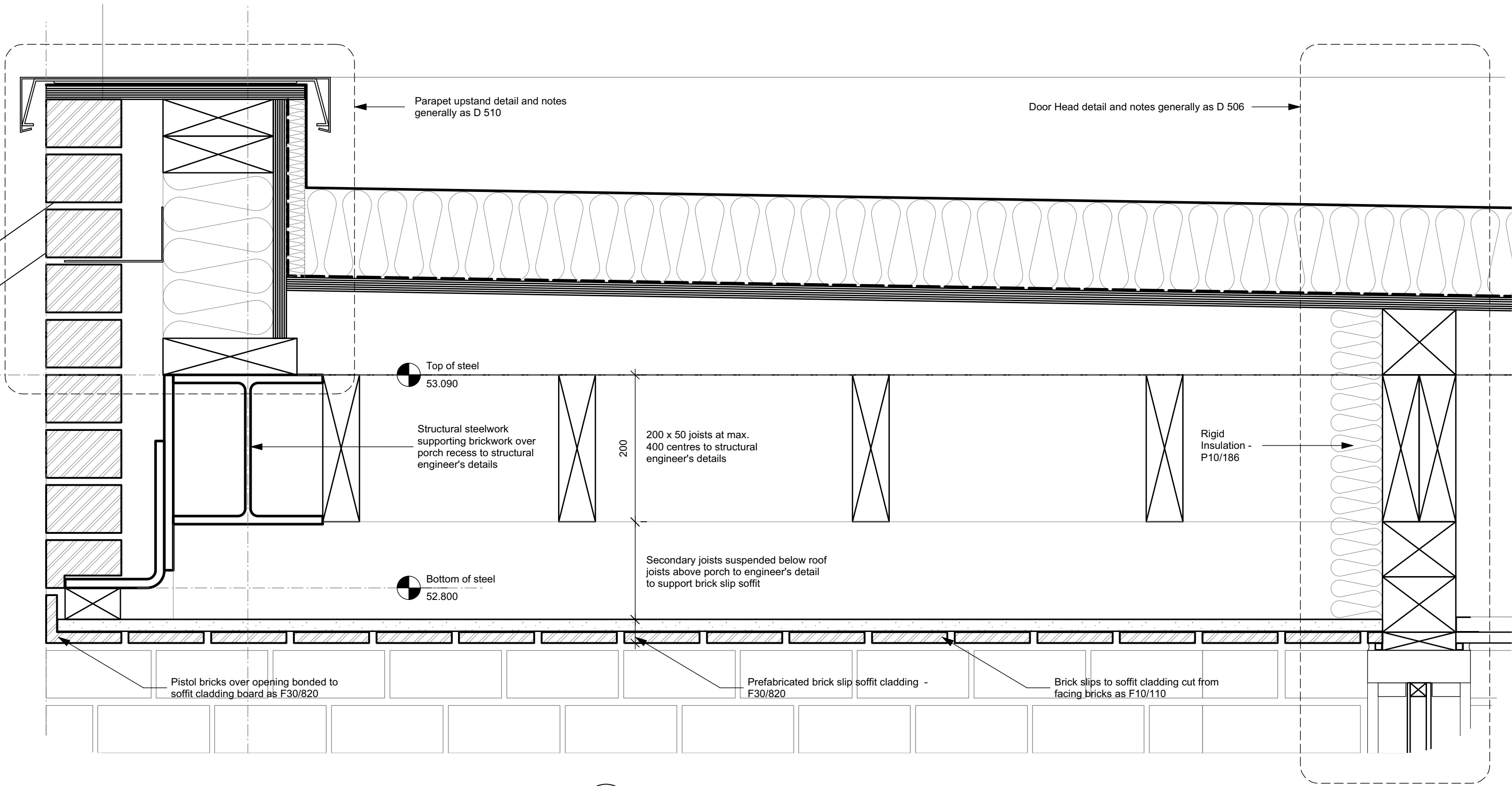
1 Entrance Soffit Detail D 511 Scale: 1:5
