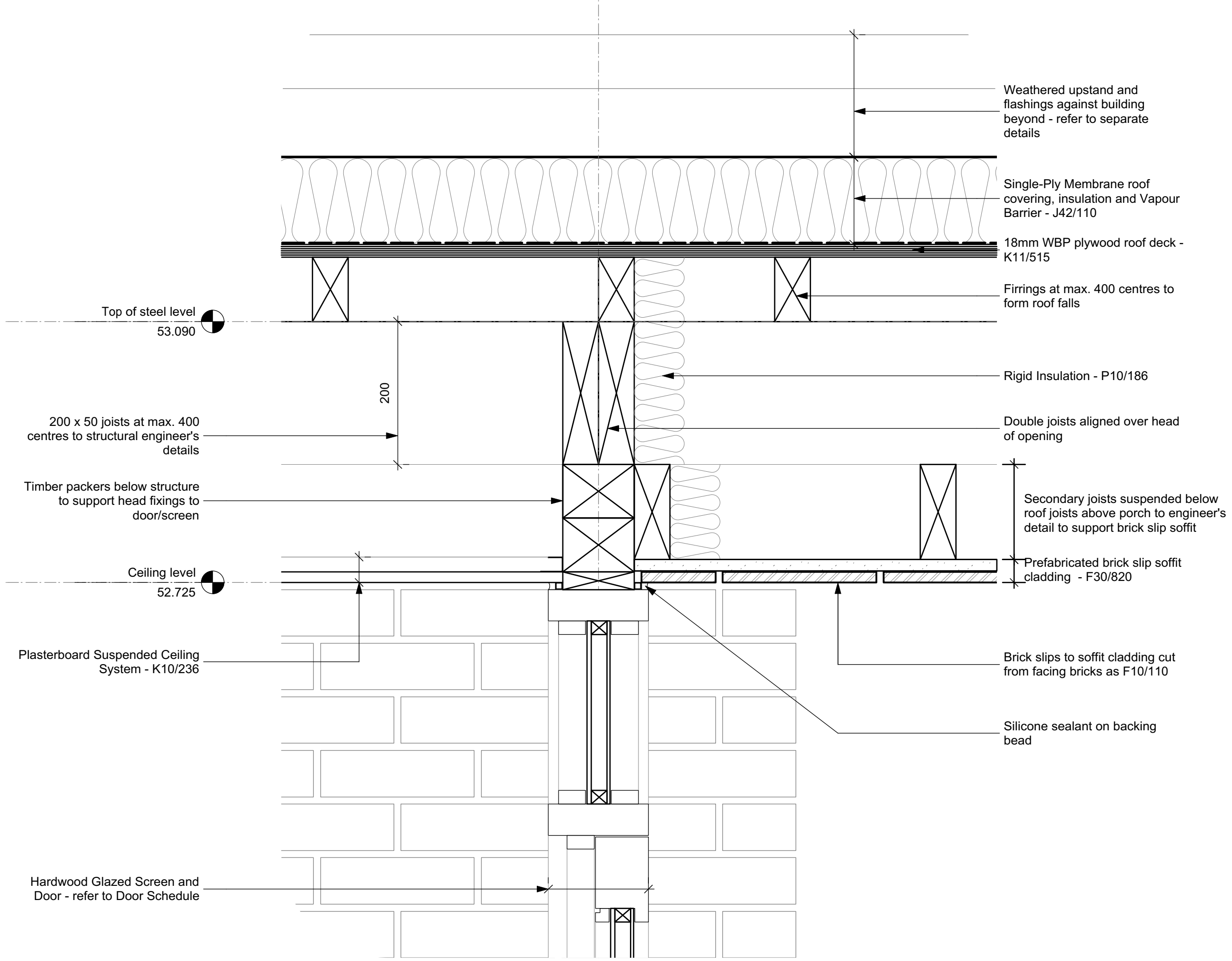
1 DG.11 Head Detail D 506 Scale: 1:5
