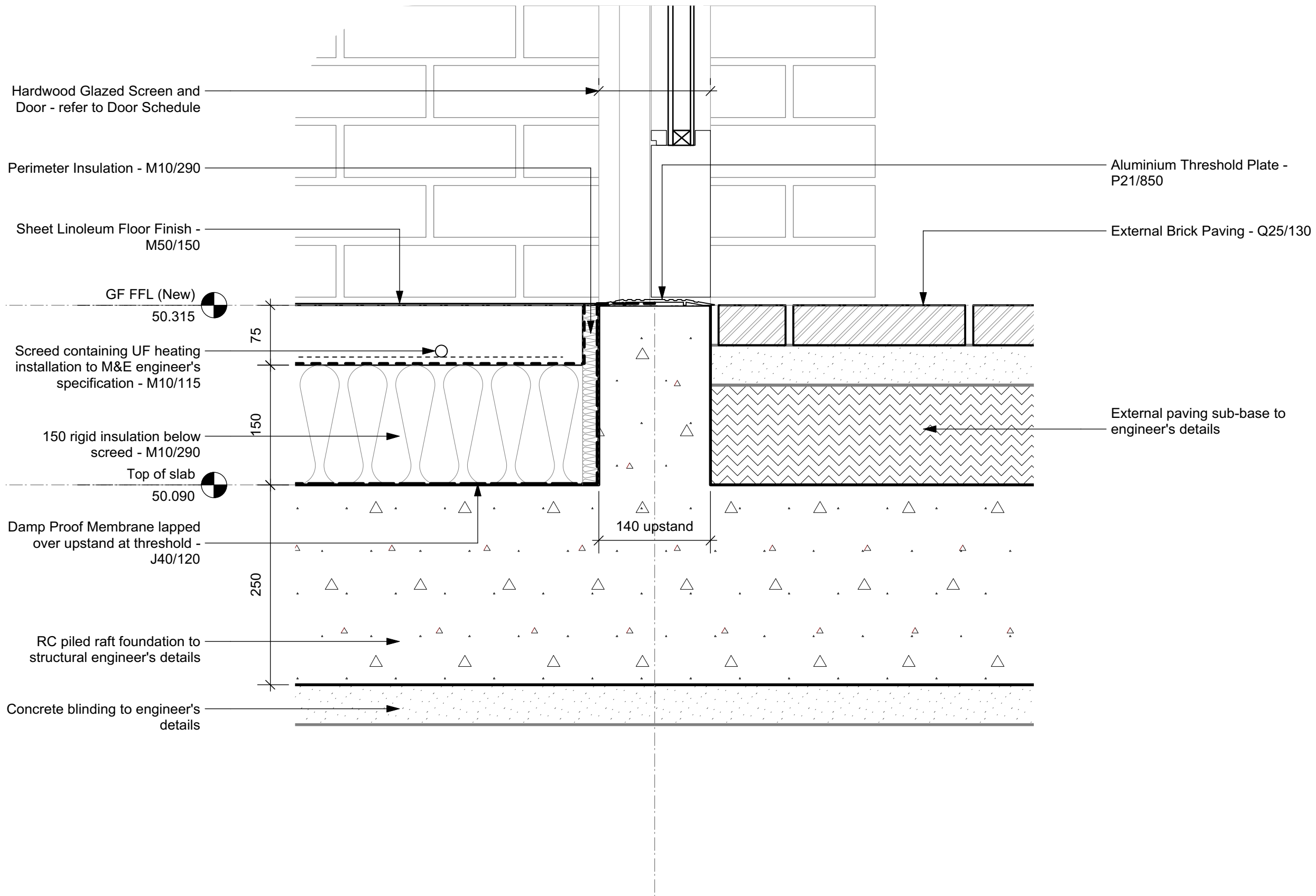
1 DG.11 Threshold Detail D 023 Scale: 1:5
