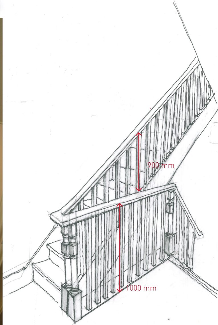
PROPOSED STAIRCASE
