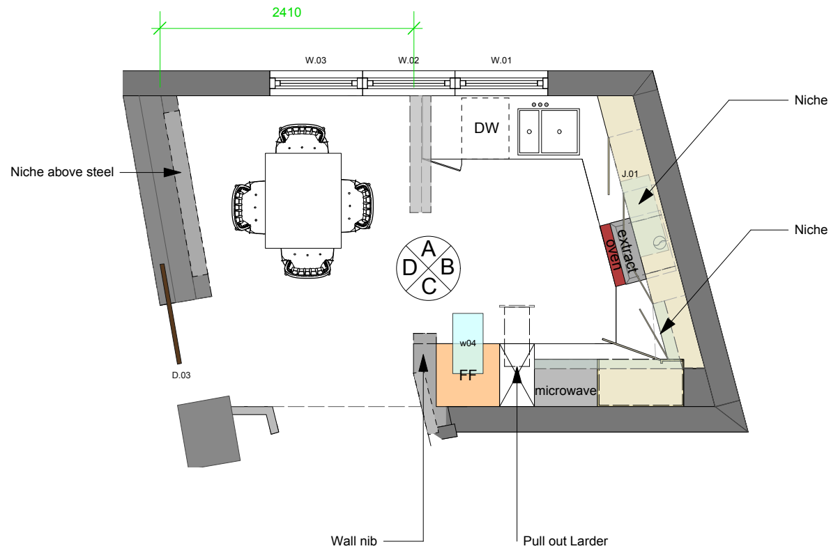
GA Floorplan 1:50 @ A3
