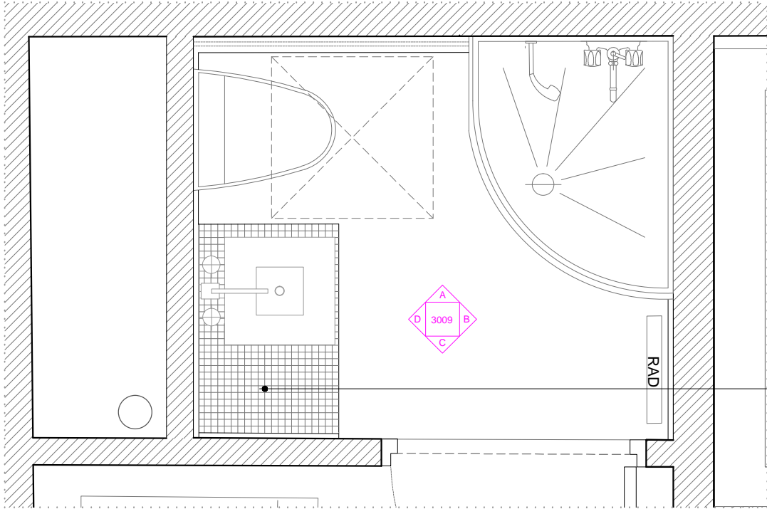
BATHROOM PLAN @1:20
