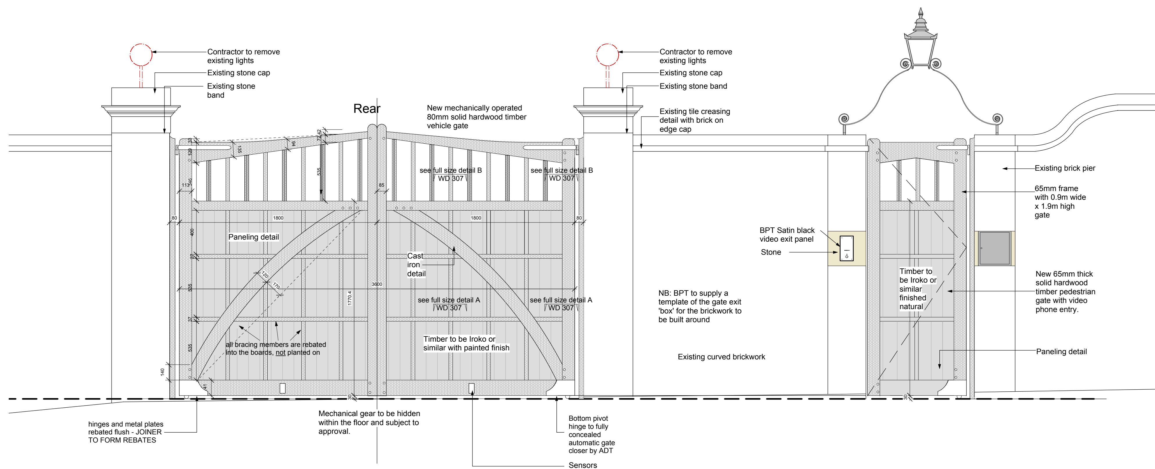
Elevation From House 1:20 Scale @A1
