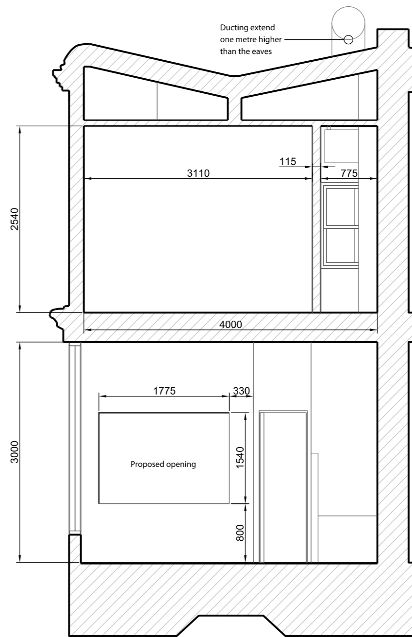
SECTION E-E
