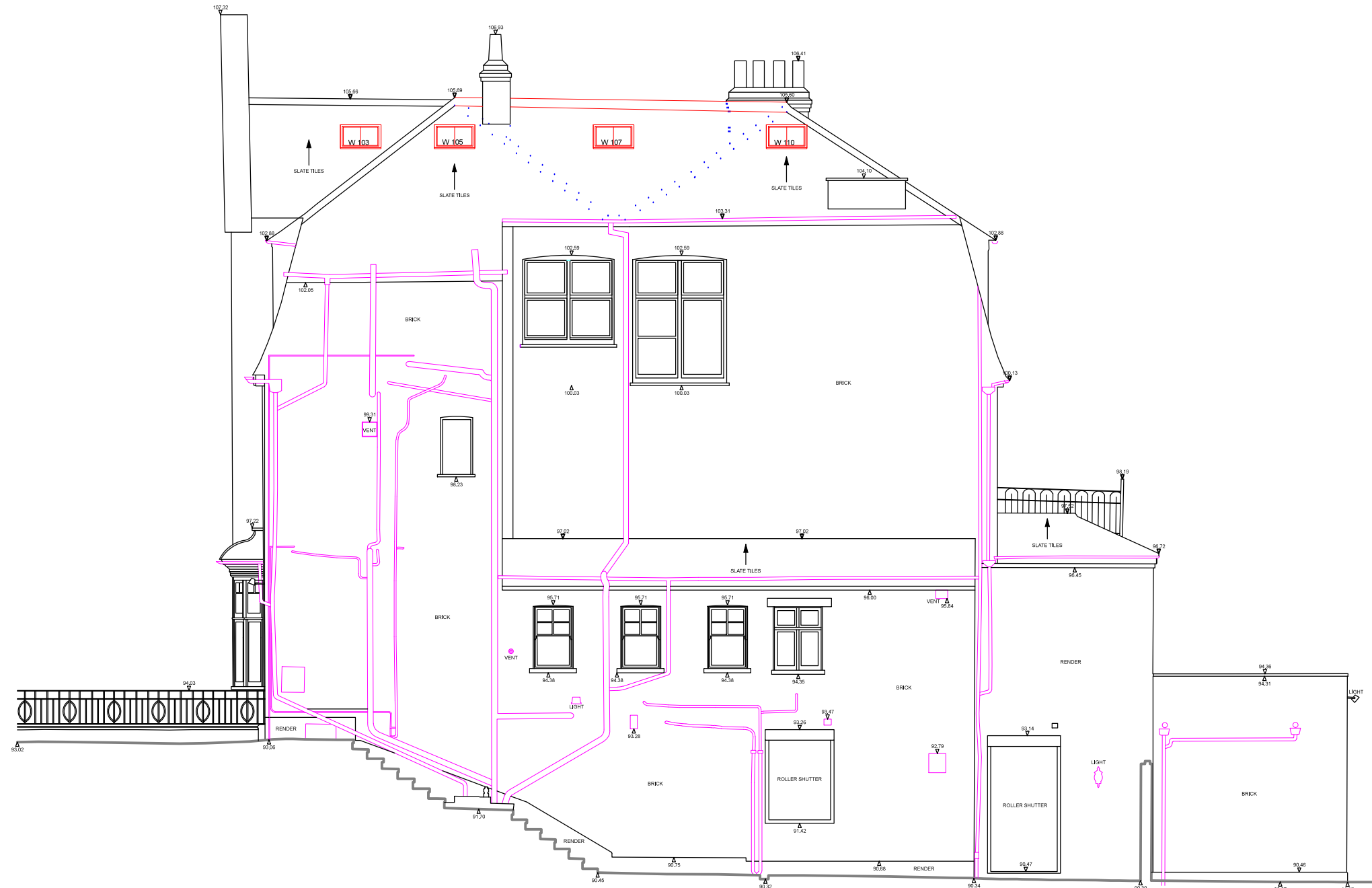
West elevation
