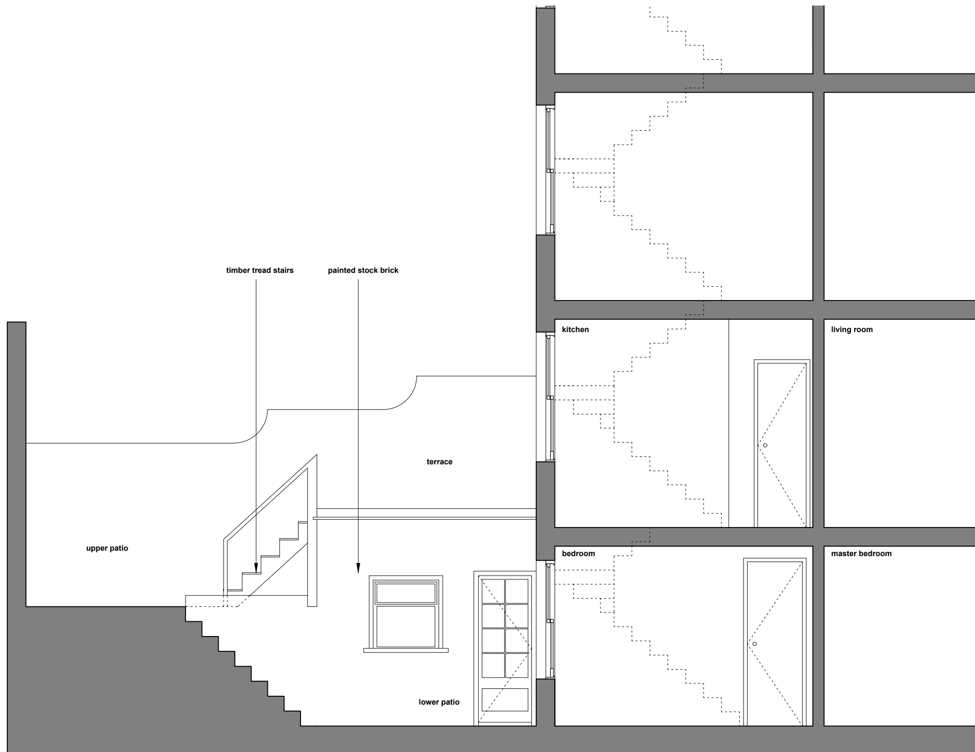
Existing rear extension elevation / section BB' . 1.50
