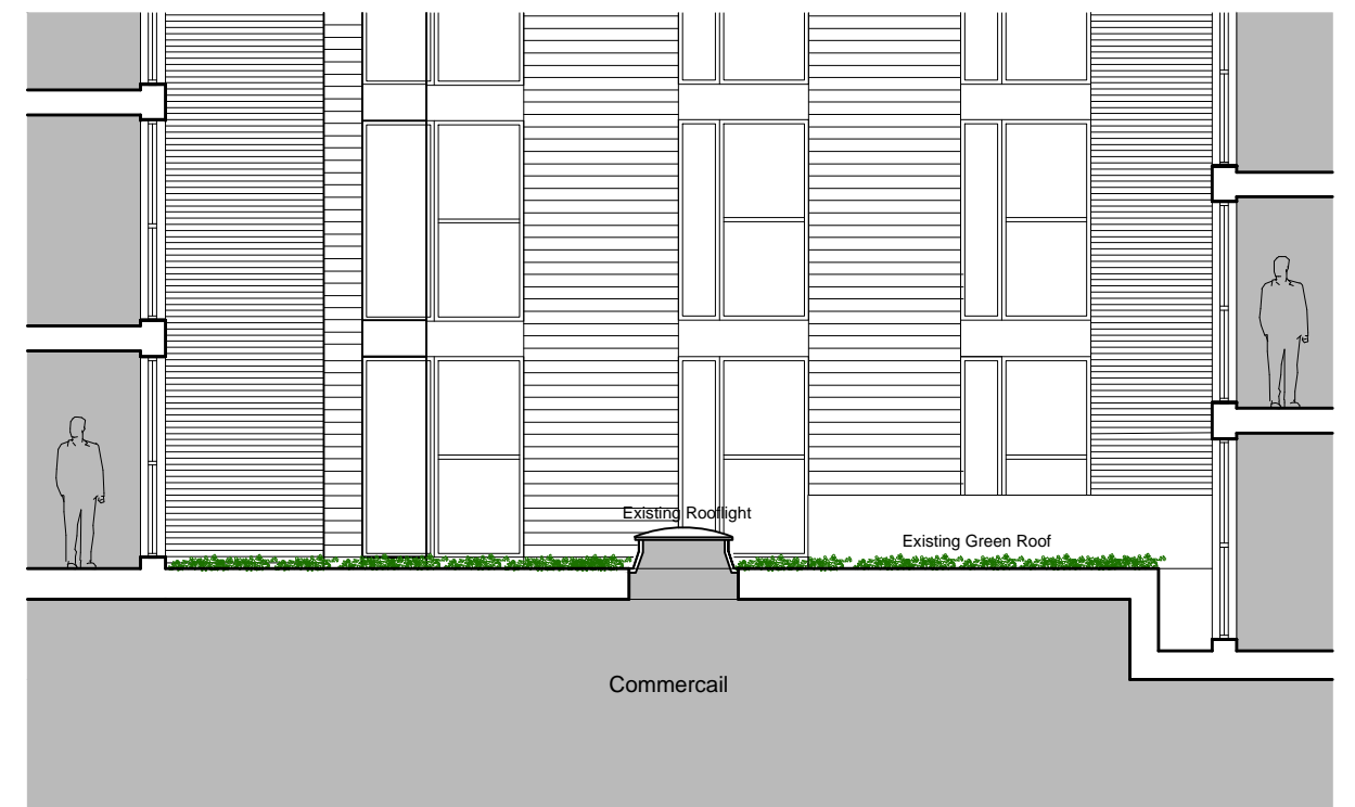
LONG SECTION YY - EXISTING
