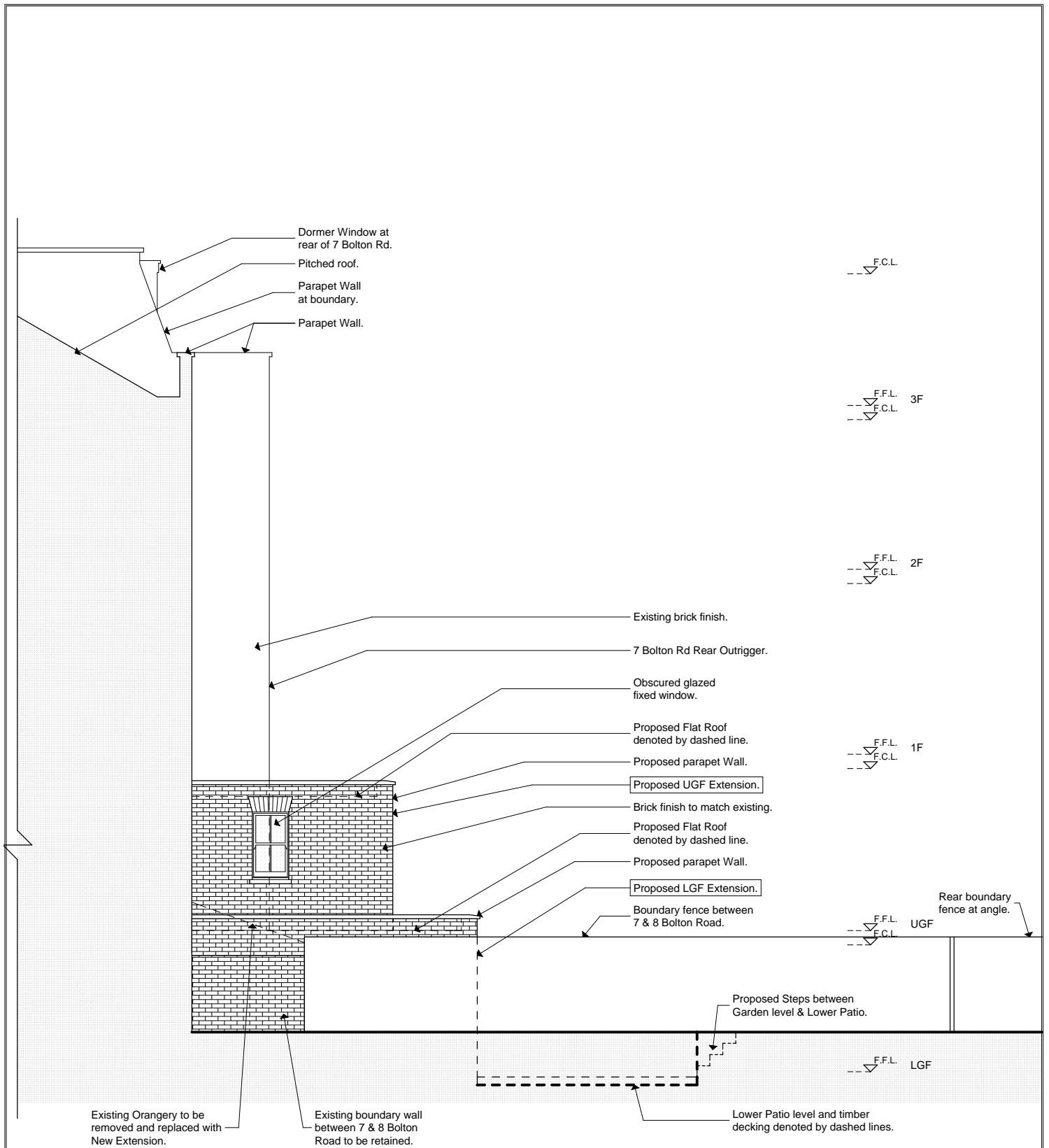
Proposed West Elevation (taken through 8 Bolton Rd)
