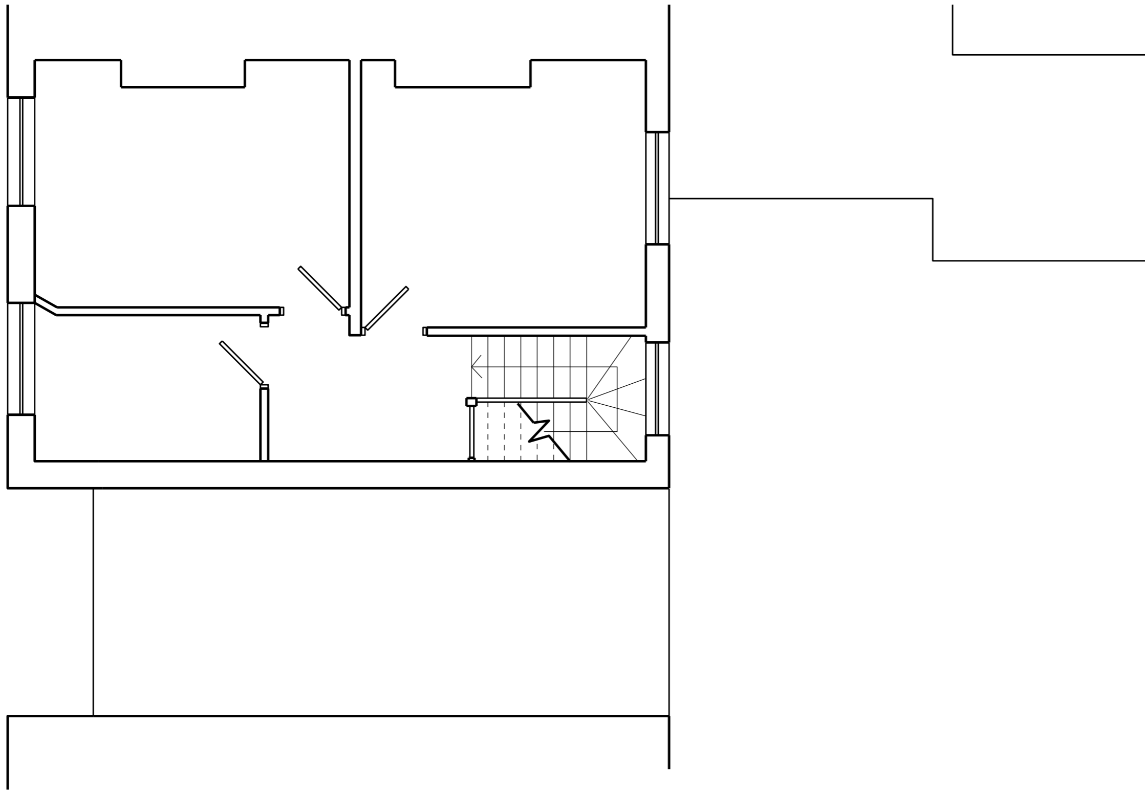
1 Second Floor Plan Existing 191_112 Scale 1:50 @ A3
