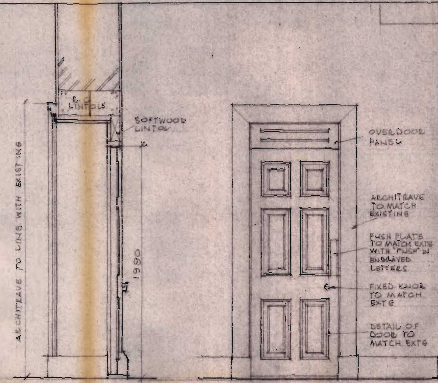
SECTION ELEVATION TO ROOM G8
