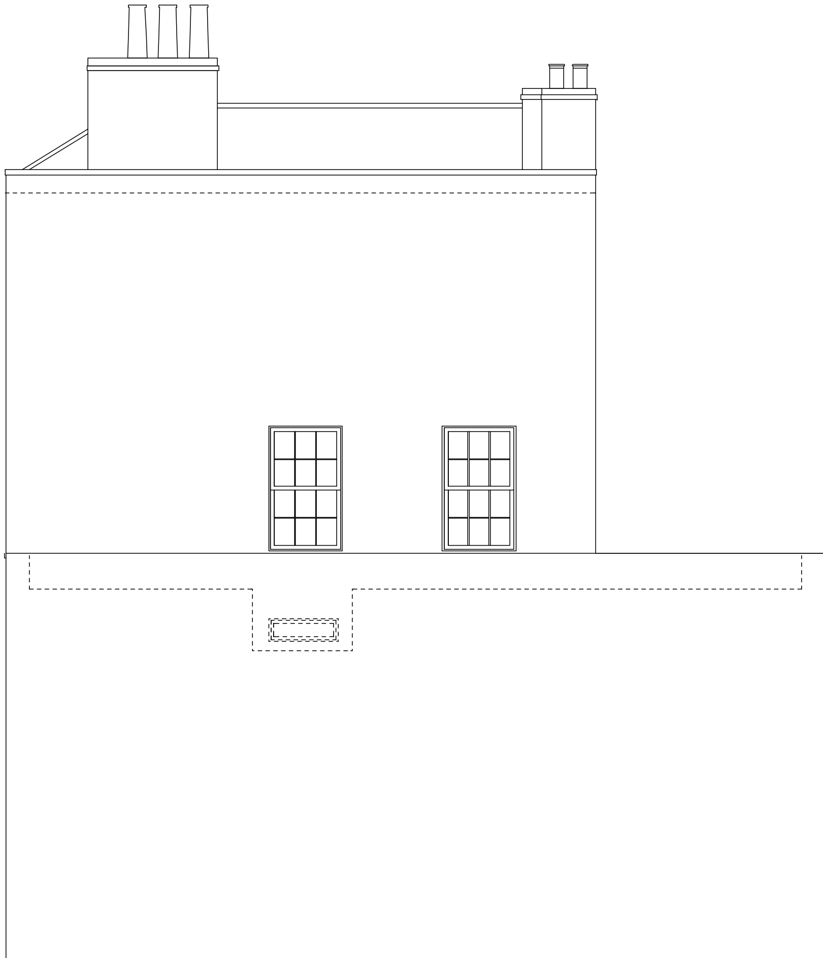
proposed south elevation Scale: 1:50
