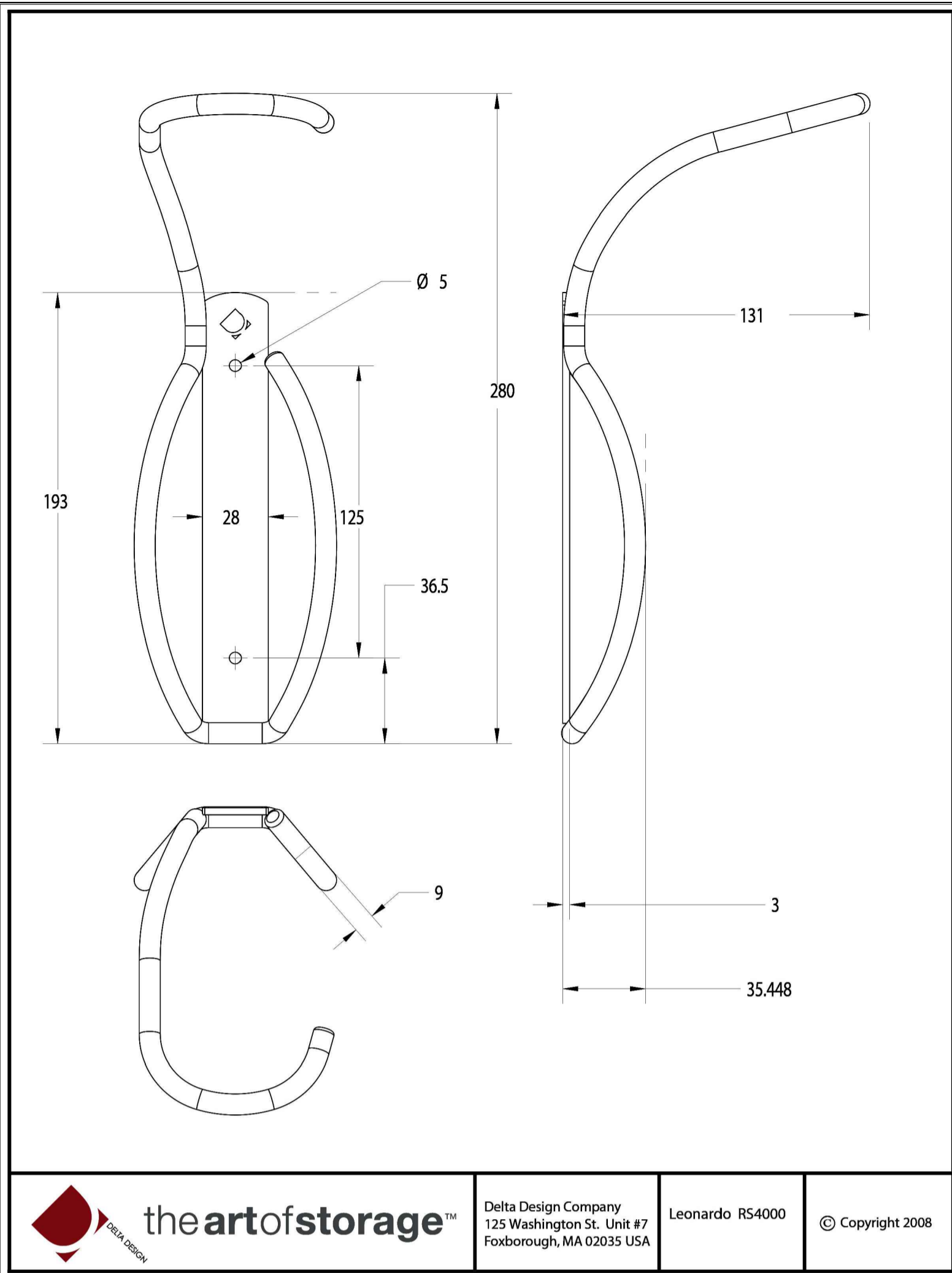
1 CYCLE RACK DETAIL 1/2
