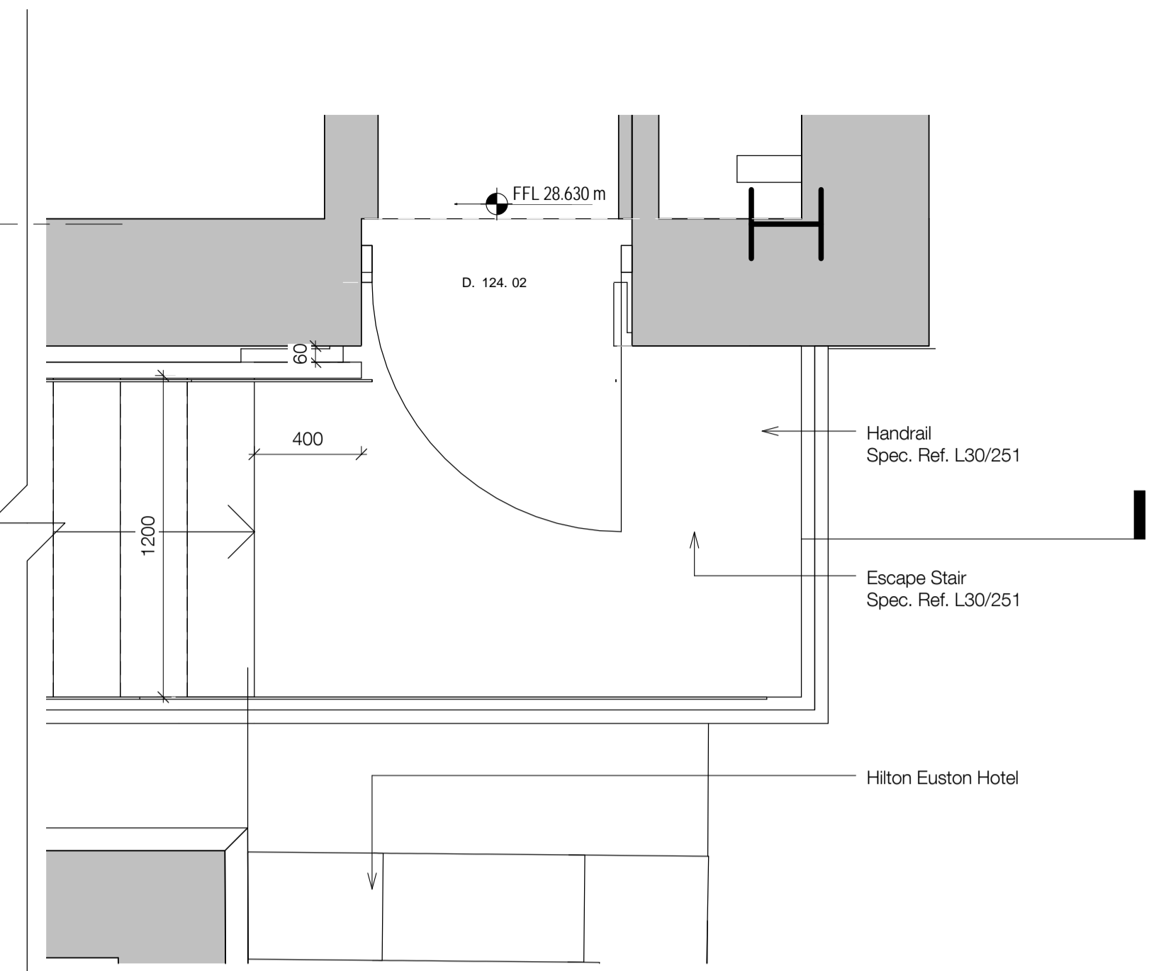
2 First Floor - Escape stairs Plan 1 : 20
