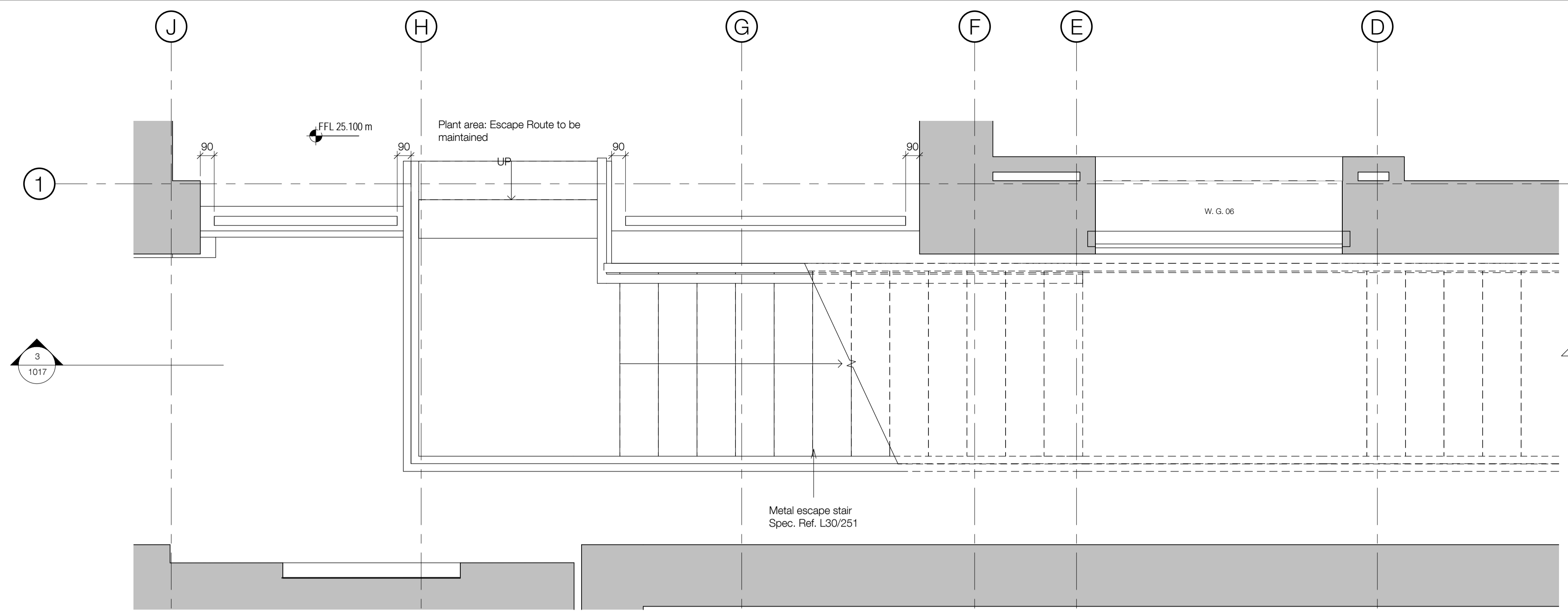
1 Ground Floor - Escape Stairs Plan 1 : 20
