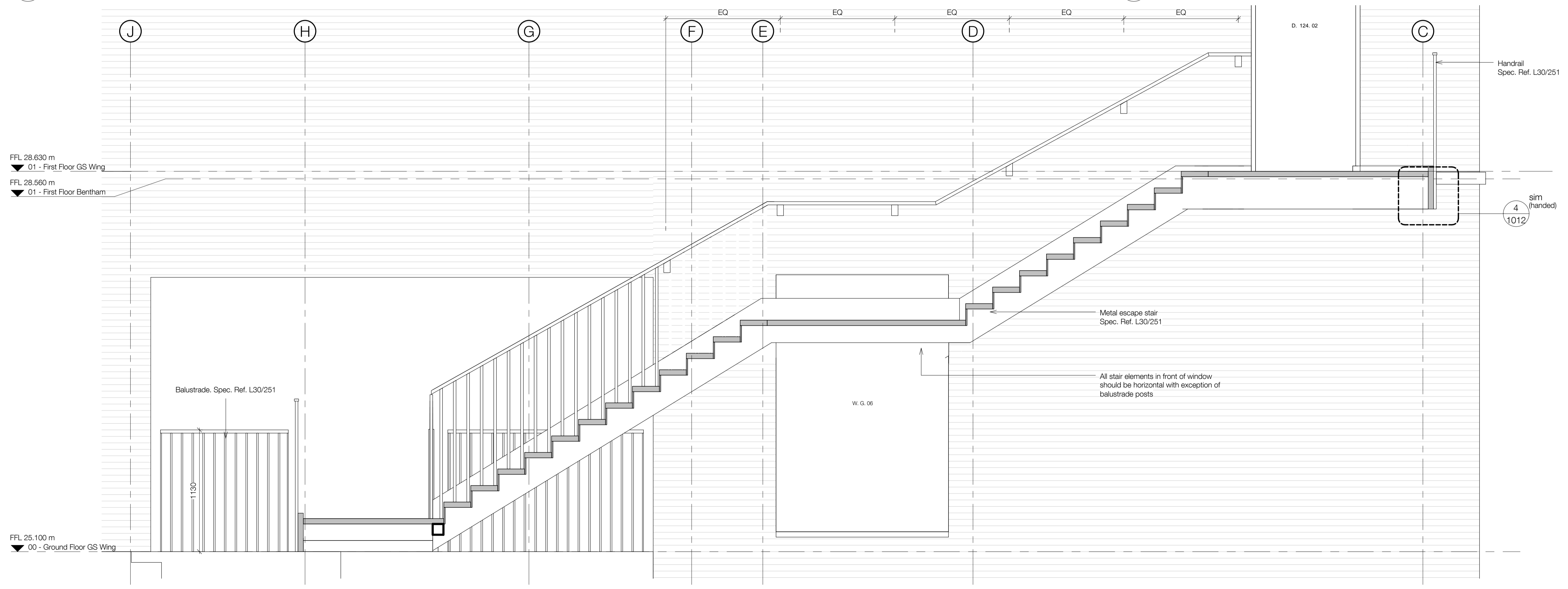
3 First Floor - Escape stair section 1 : 20
