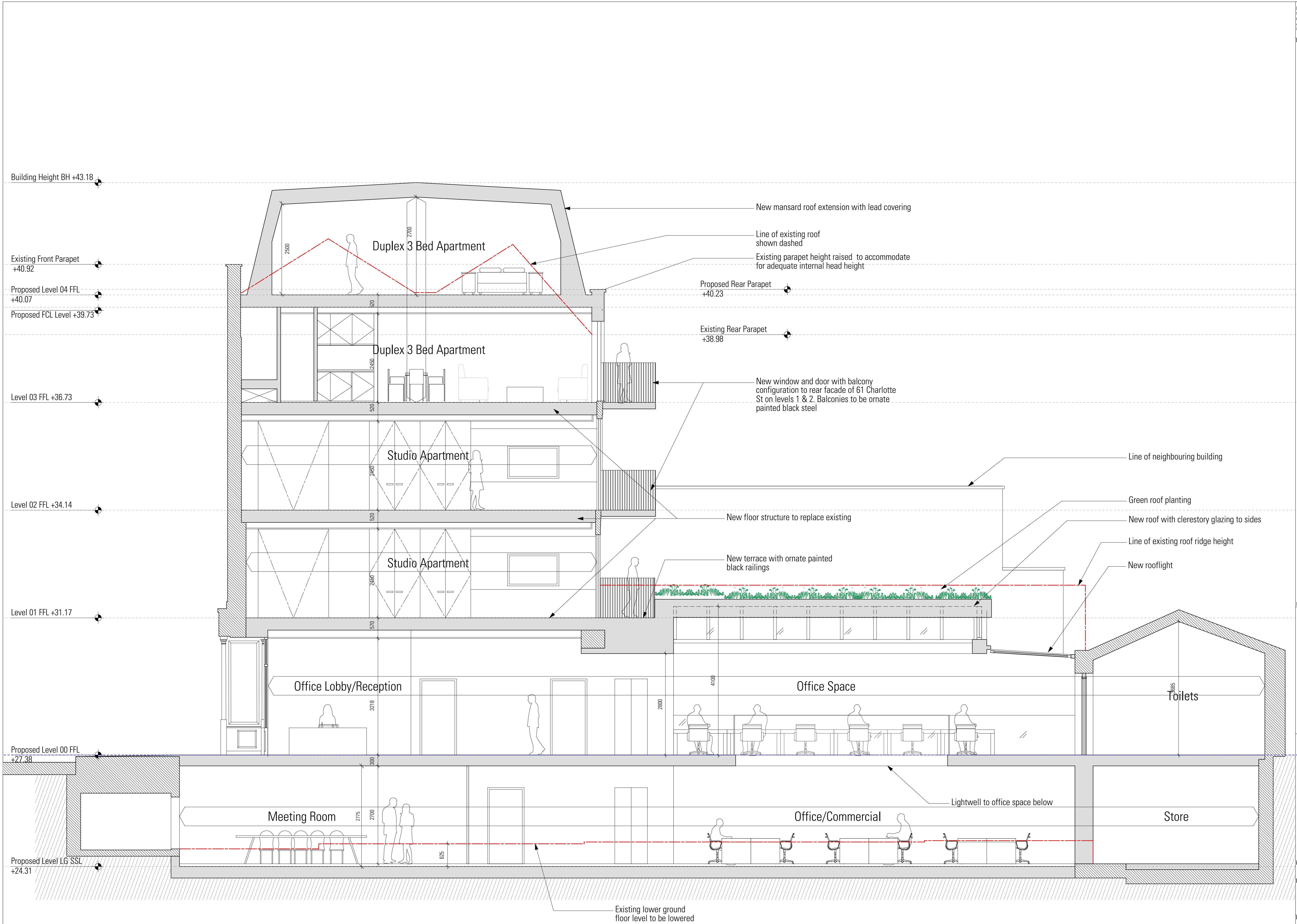
01 Proposed Section A-A Scale 1:50@A1, 1:100@A3
