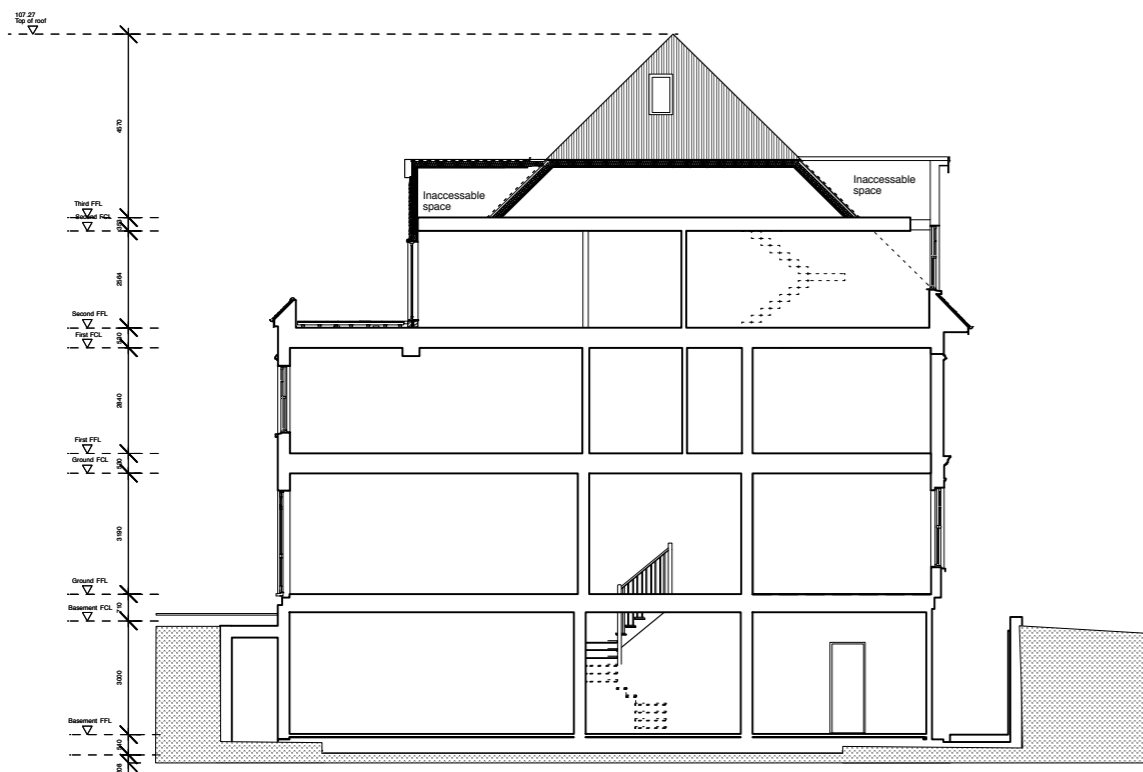
APPROVED SECTION
