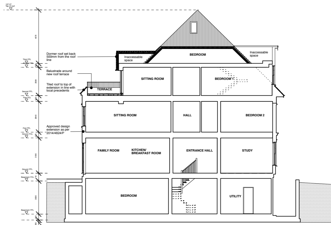
PROPOSED SECTION
