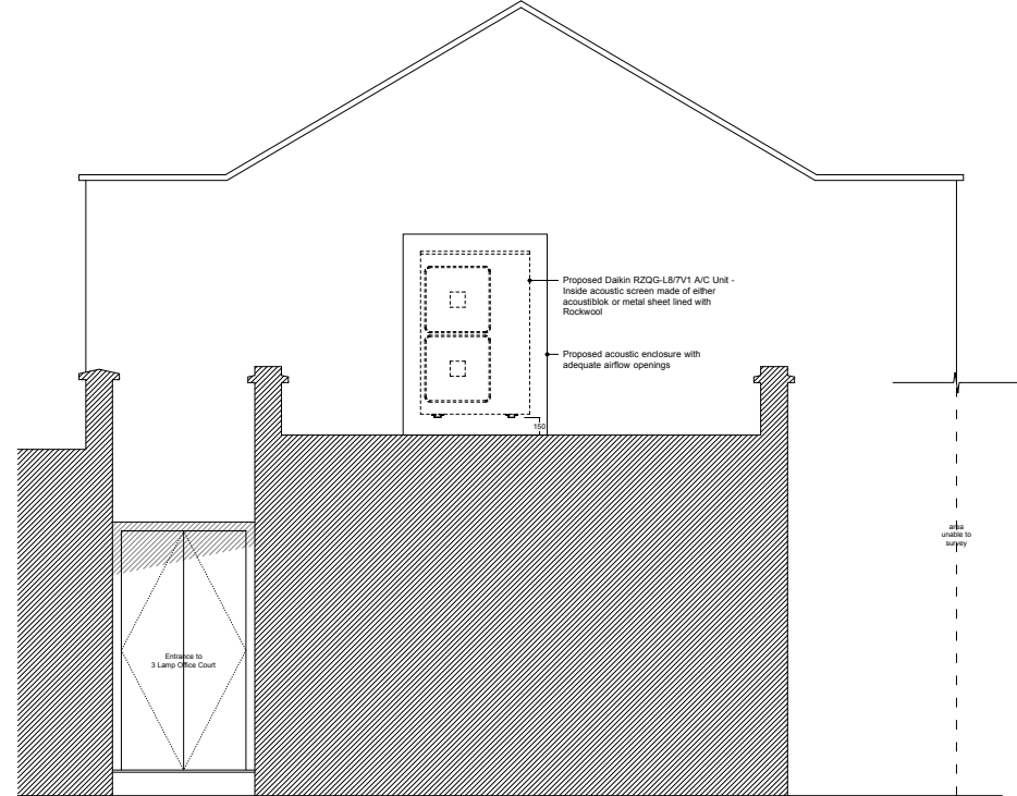
3 EAST ELEVATION 1:50
