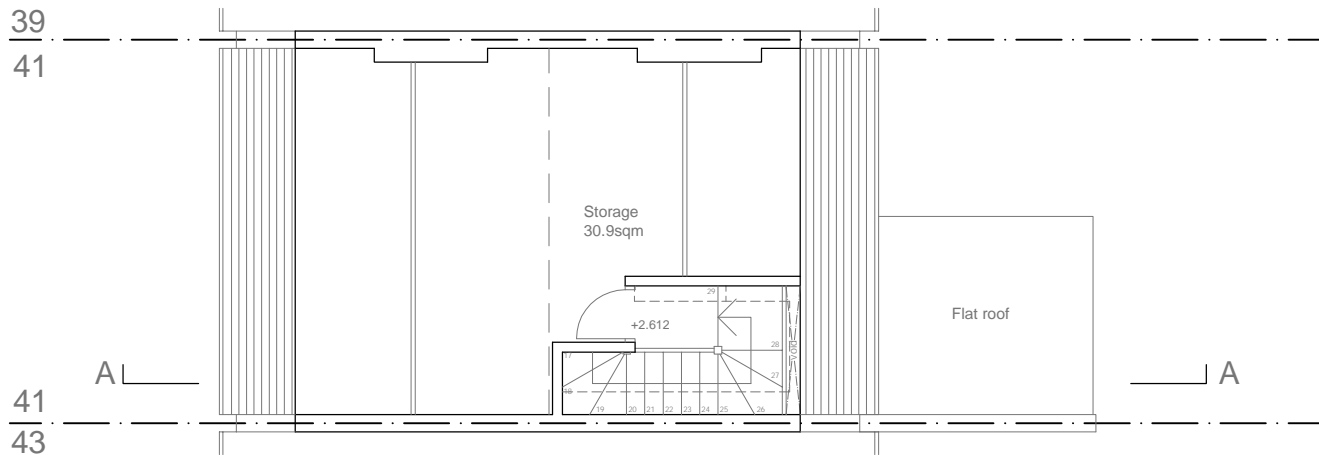
Proposed Loft Floor Plan Floor Area 37sqm
