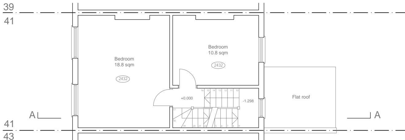
Proposed Second Floor Plan Floor Area 37sqm
