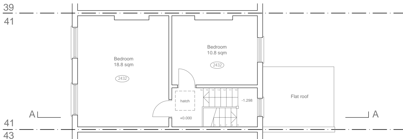
Existing Second Floor Plan Floor Area 37sqm
