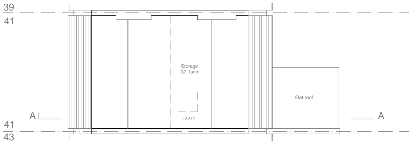
Existing Loft Floor Plan Floor Area 37sqm
