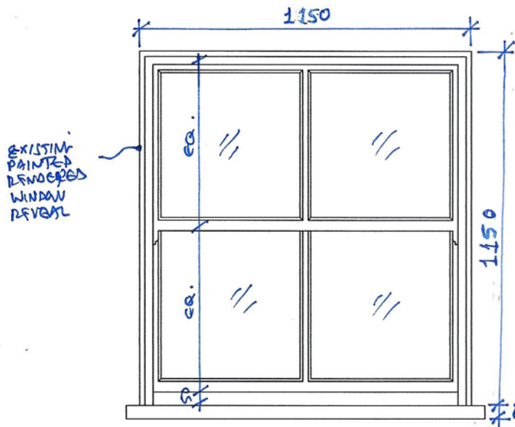
ELEVATION (EXTERNAL)
