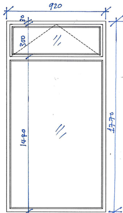
ELEVATION (EXTERNAL)
